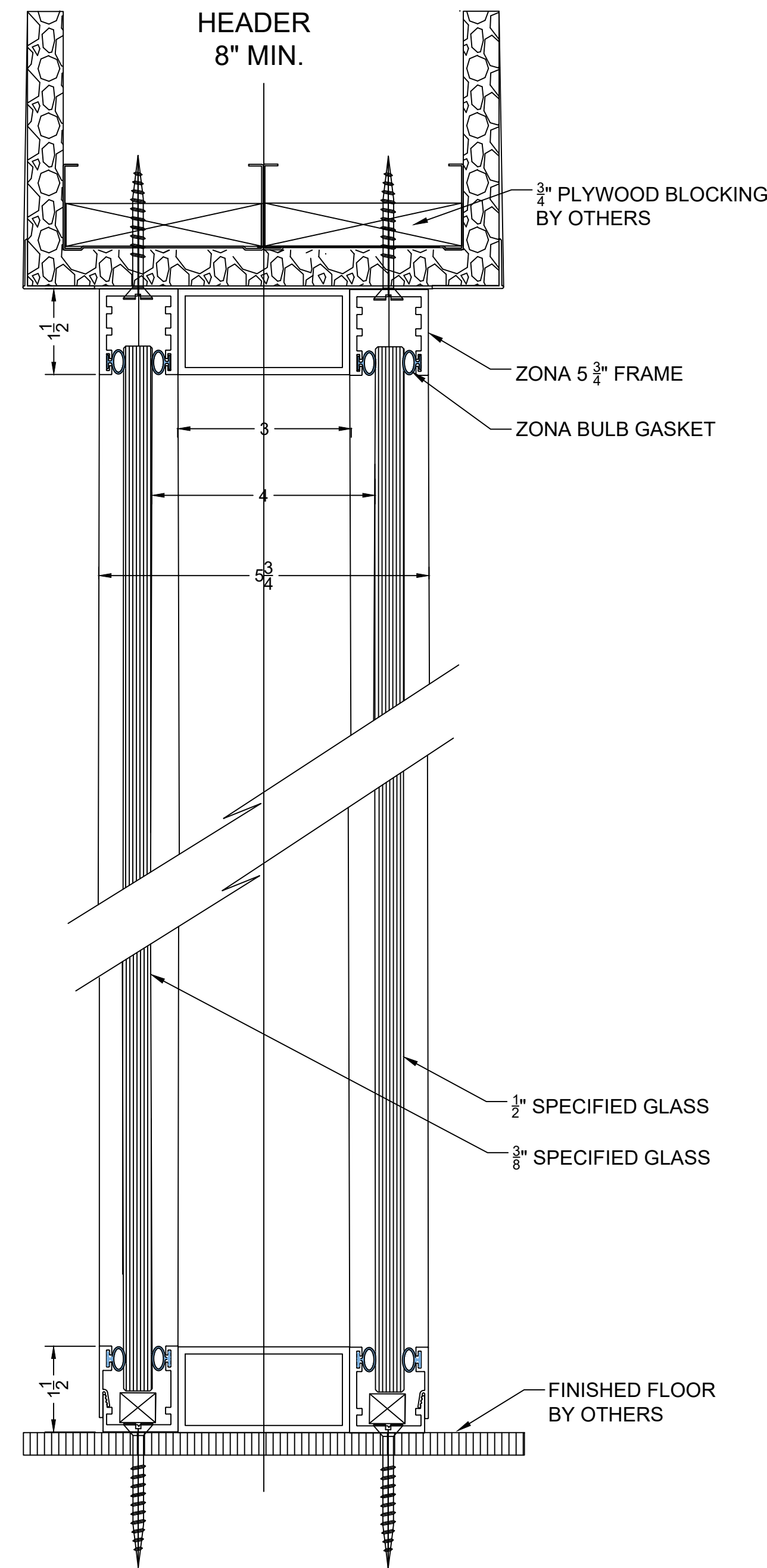
1 MAX. STC = 51 VERT. SECT @ ZONA DBL GLZD FIXED PANEL
