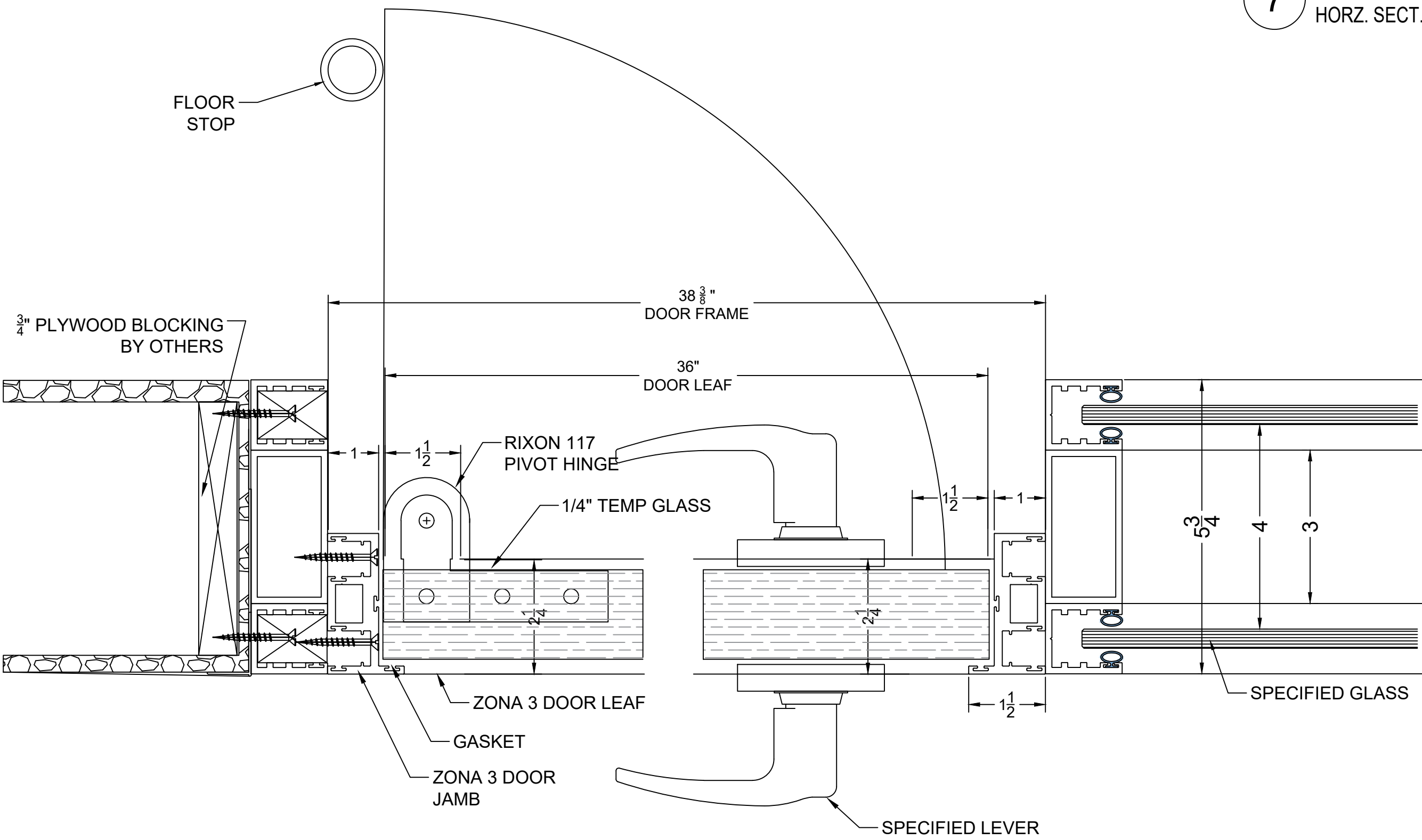
6A DOOR @ NIB WALL HORZ. SECT. @ WOOD DOOR W/LOCKSET 51 STC
