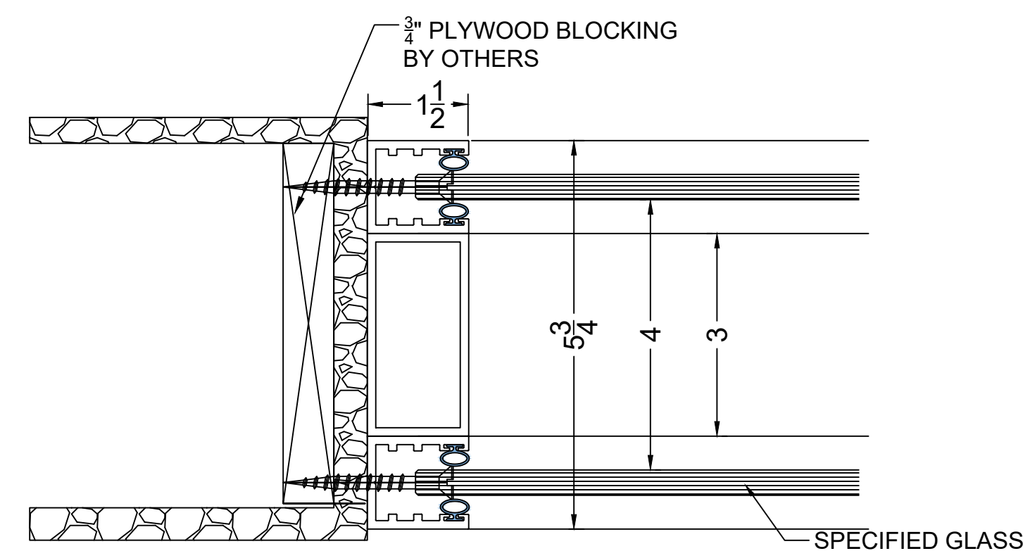
3 SECTION @ FIXED PANEL @ WALL 51 STC
