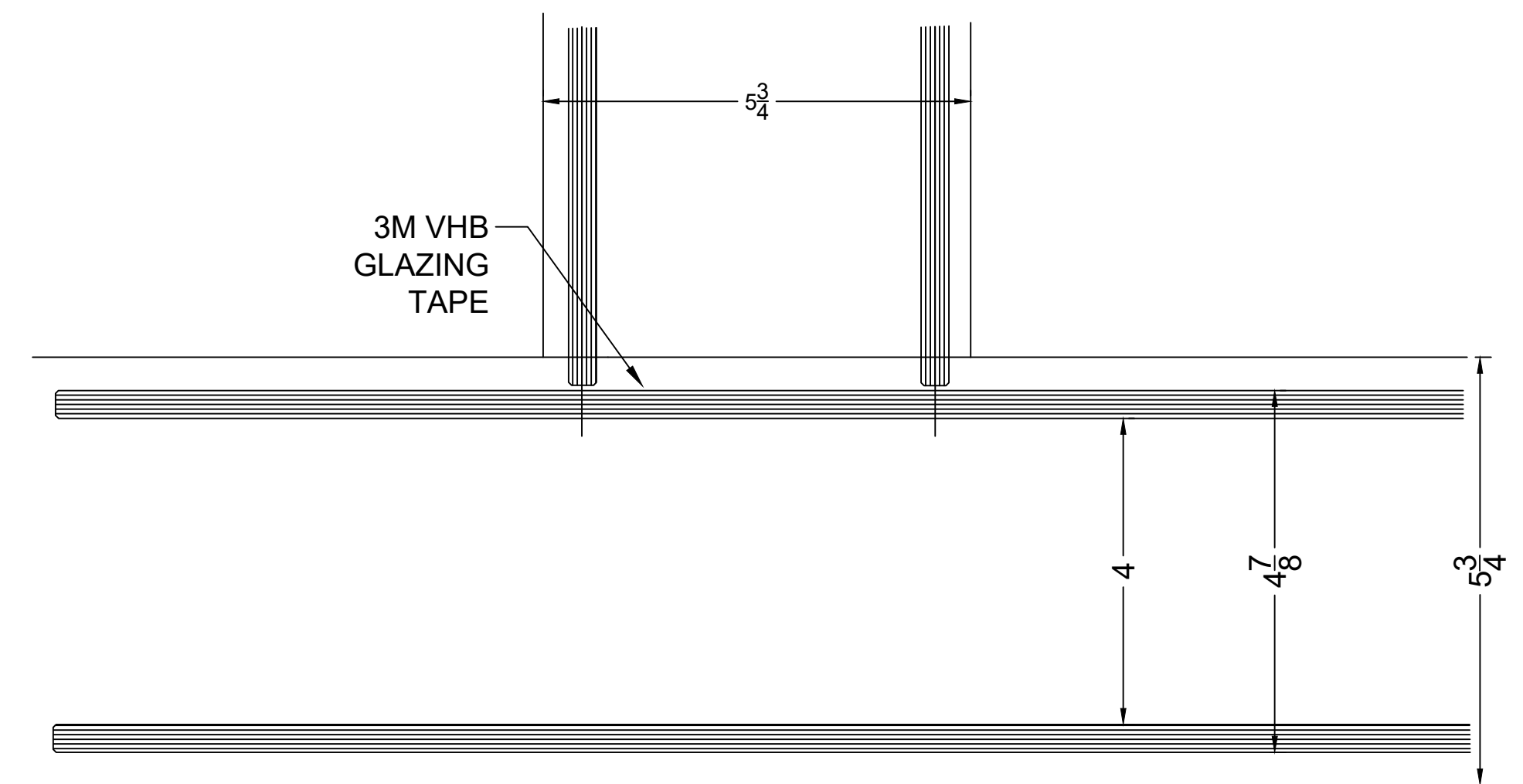
4 HORZ. SECT @ "T" CONNECTION 51 STC
