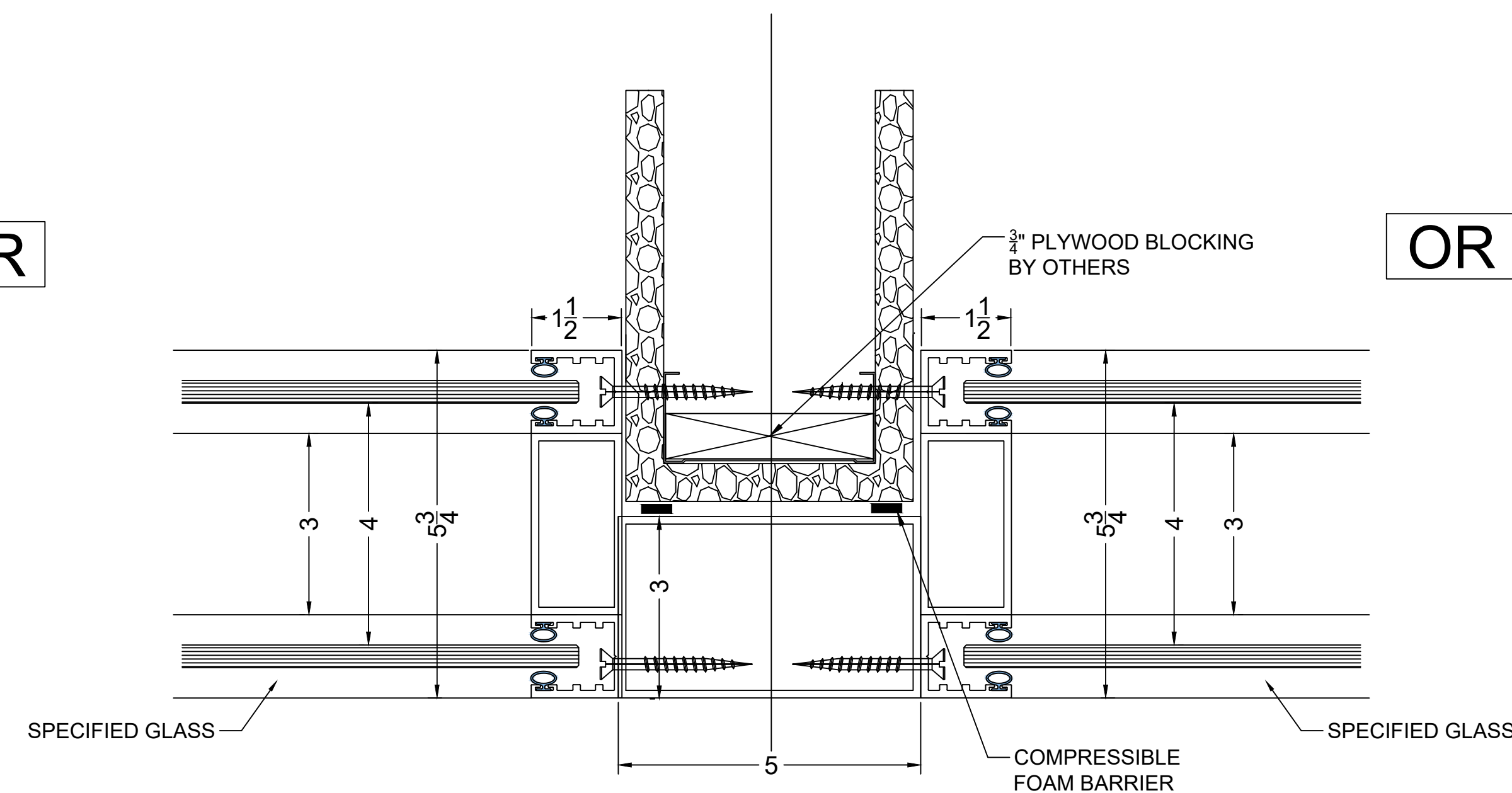
4 HORZ. SECT @ DIVIDER WALL WITH FLY-BY POST 51 STC
