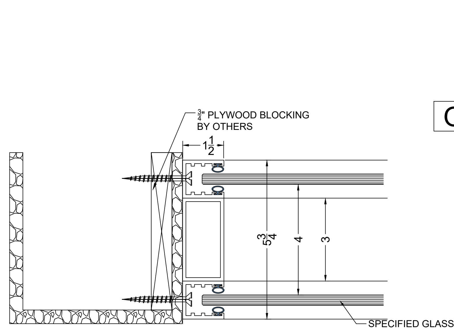
4 SECTION @ FIXED PANEL @ DIVIDER WALL 51 STC
