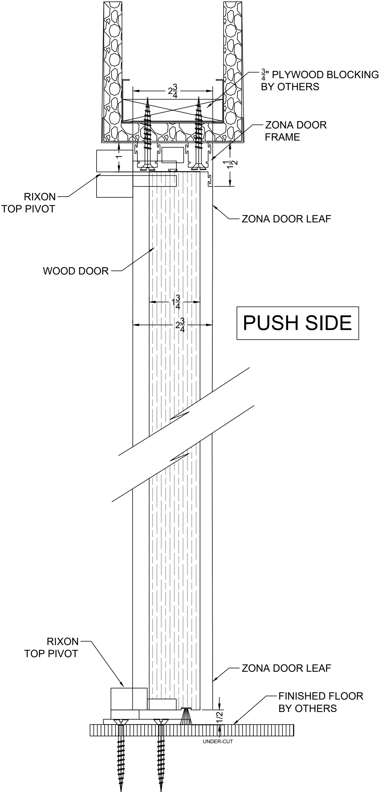
2A RIXON PIVOT HINGE- FREE-SWING DOOR VERT. SECT. @ WOOD DOOR
