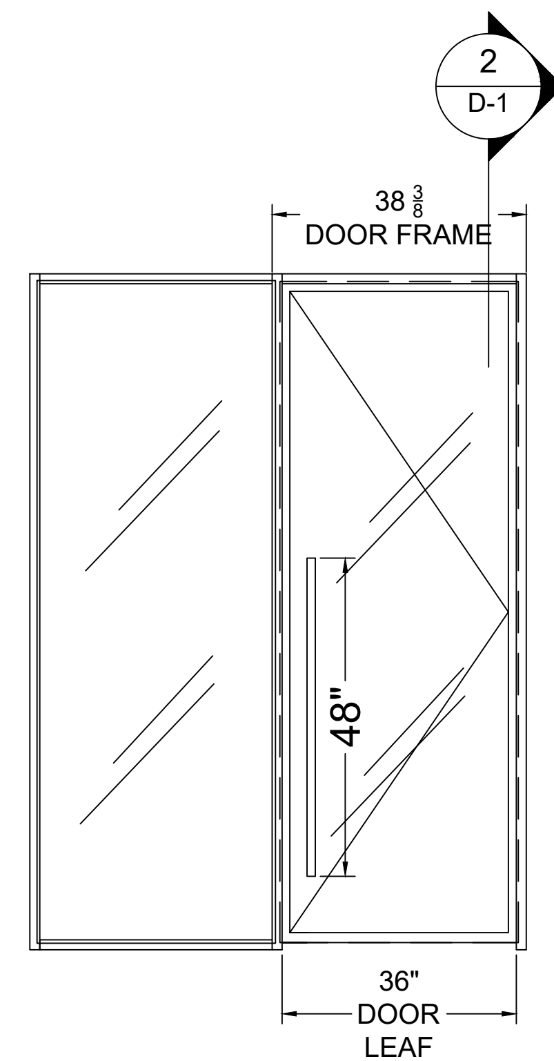
51 DOOR WITH FIXED GLASS
