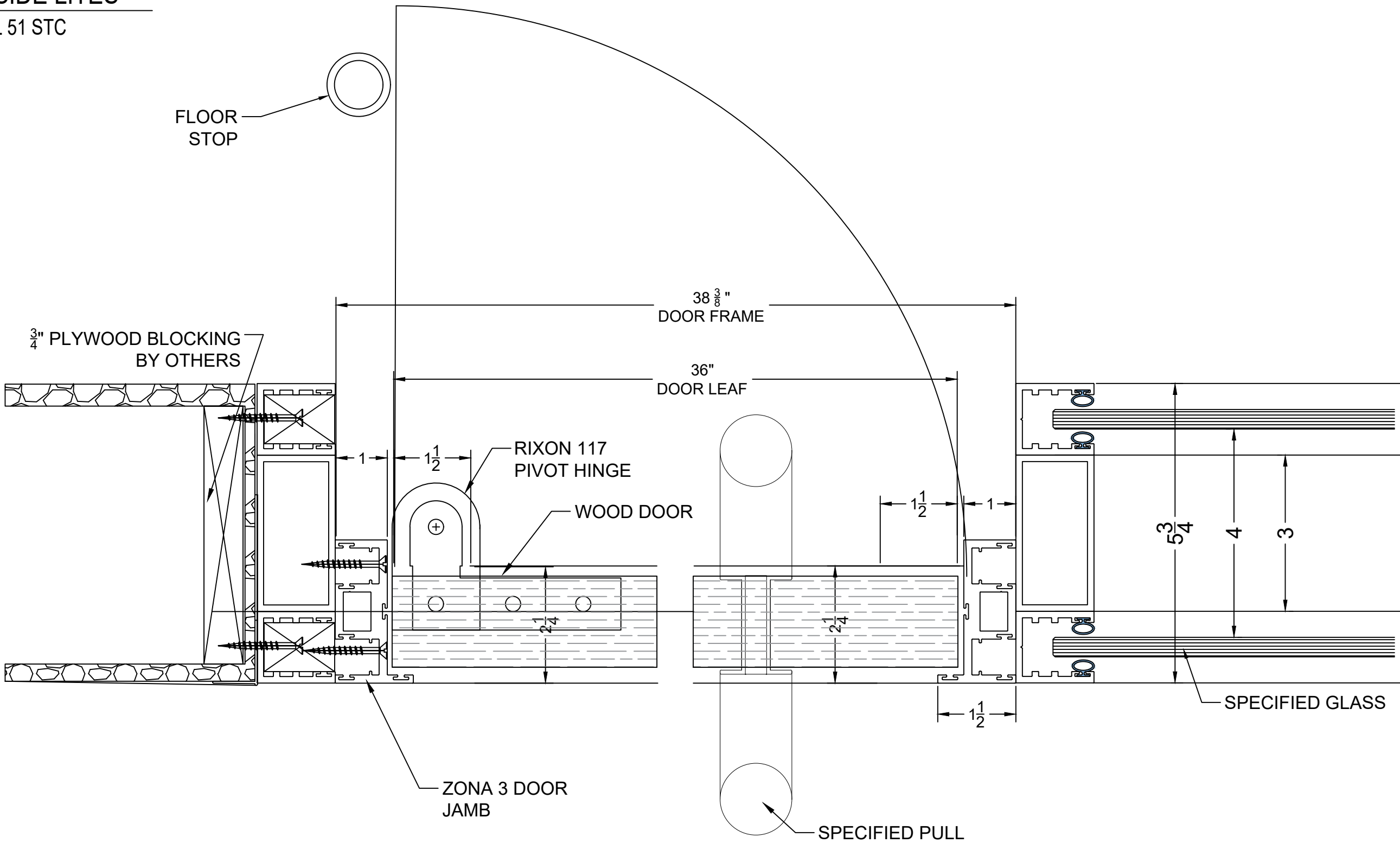
5A DOOR @ NIB WALL HORZ. SECT. @ WOOD DOOR W/PULL 51 STC
