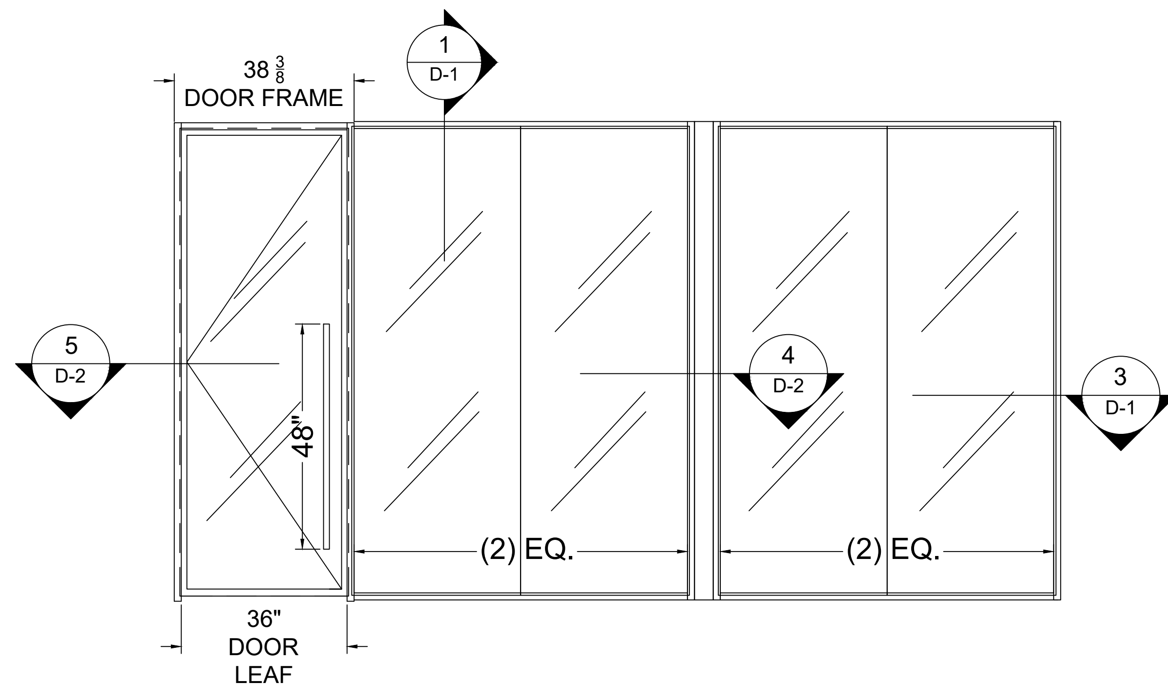
51 TYPICAL SYSTEM W/ DOOR STARTER AND DIVIDER EXAMPLE
