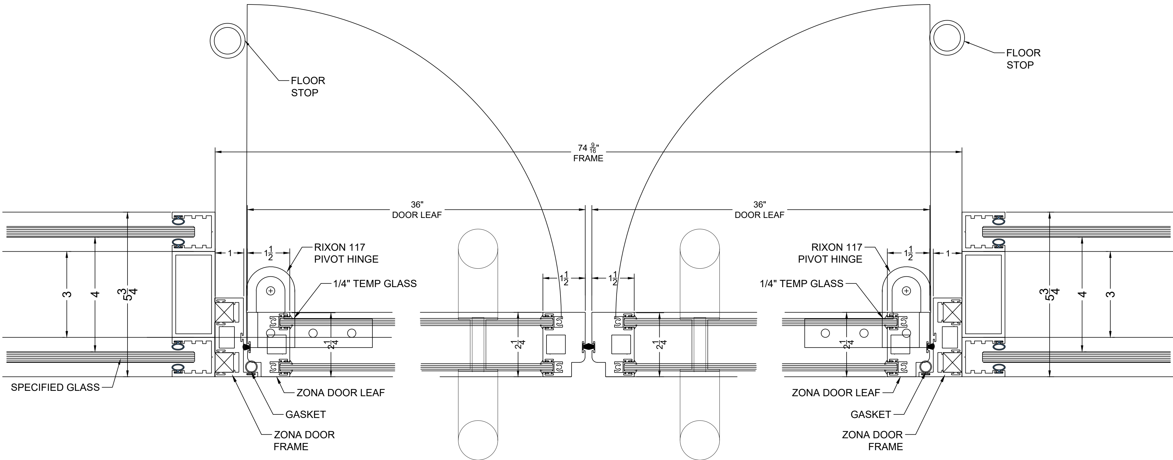
7 (2) ACTIVE DOORS BTW FIXED GLASS SIDE LITES HORZ. SECT. @ DBL GLZD DOUBLE DOORS W/PULL 51 STC
