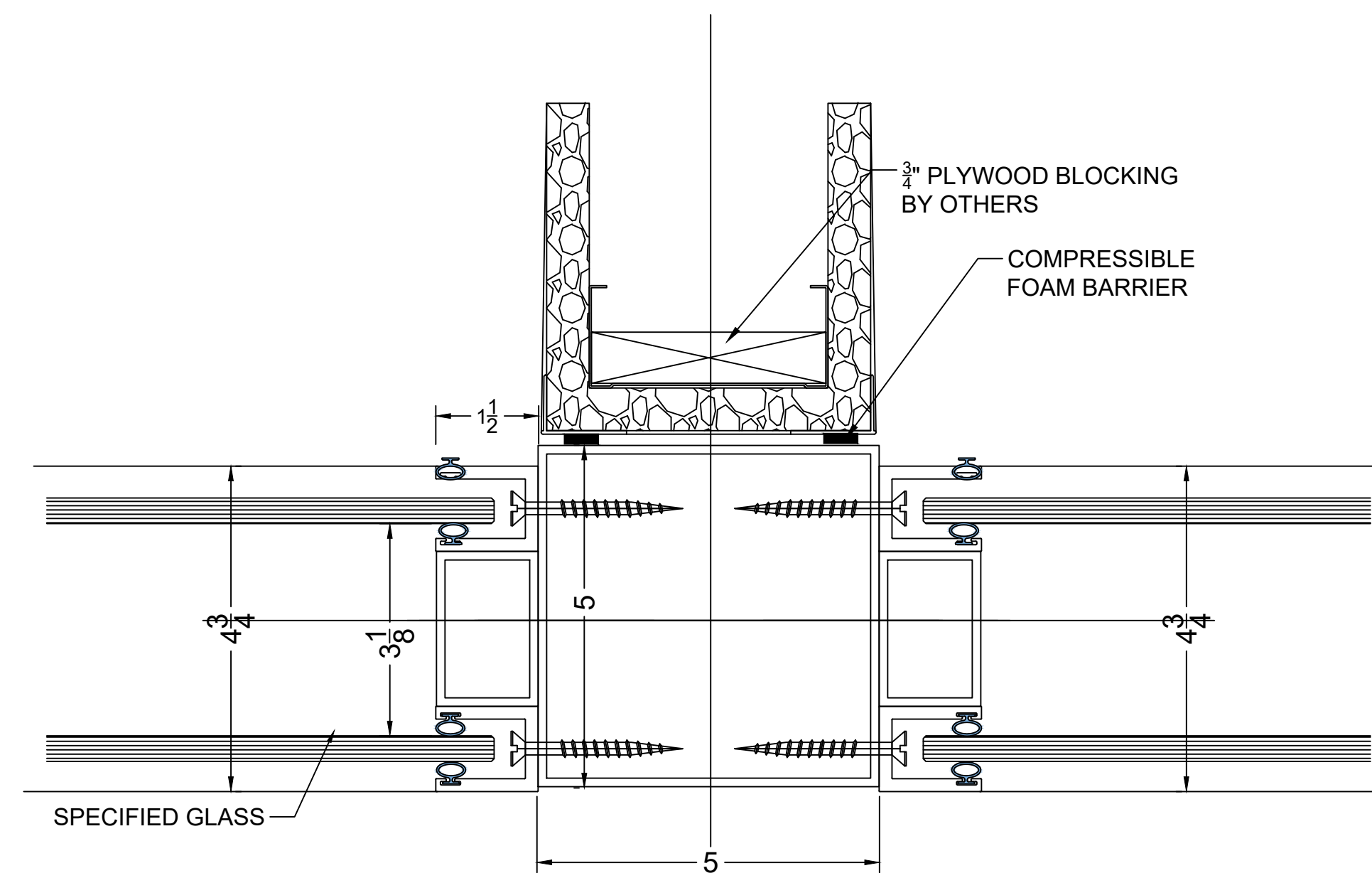
4 HORZ. SECT @ DIVIDER WALL WITH FLY-BY POST 49 STC
