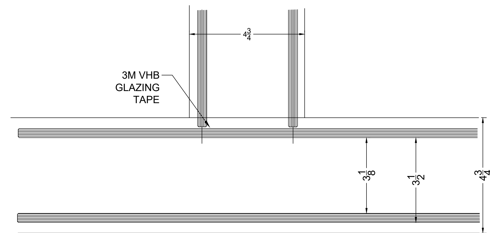
4 HORZ. SECT @ "T" CONNECTION 49 STC
