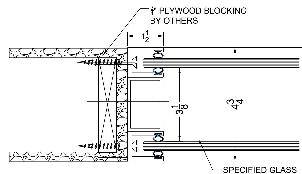
3 SECTION @ FIXED PANEL @ WALL 49 STC
