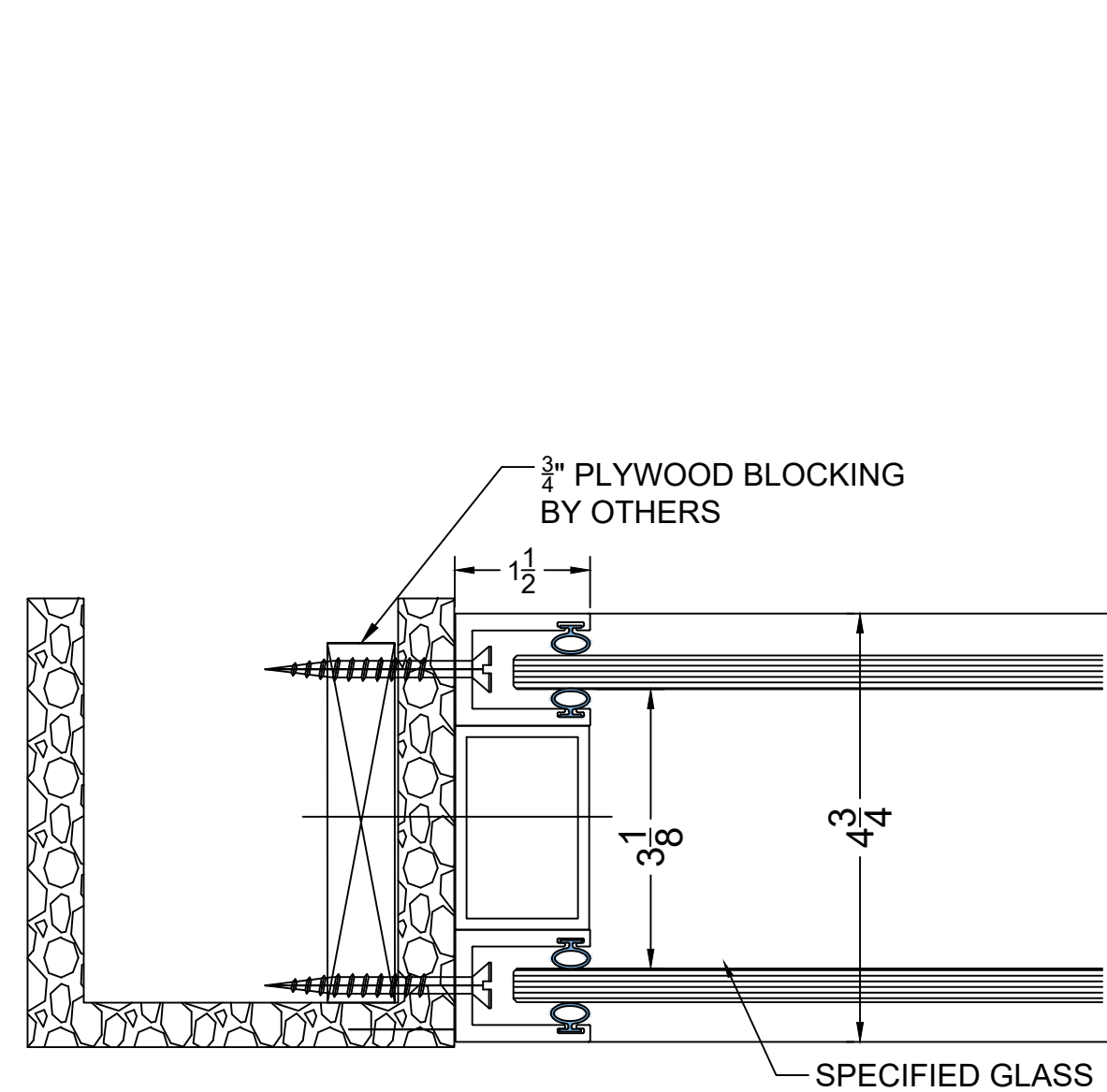
4 SECTION @ FIXED PANEL @ DIVIDER WALL 49 STC
