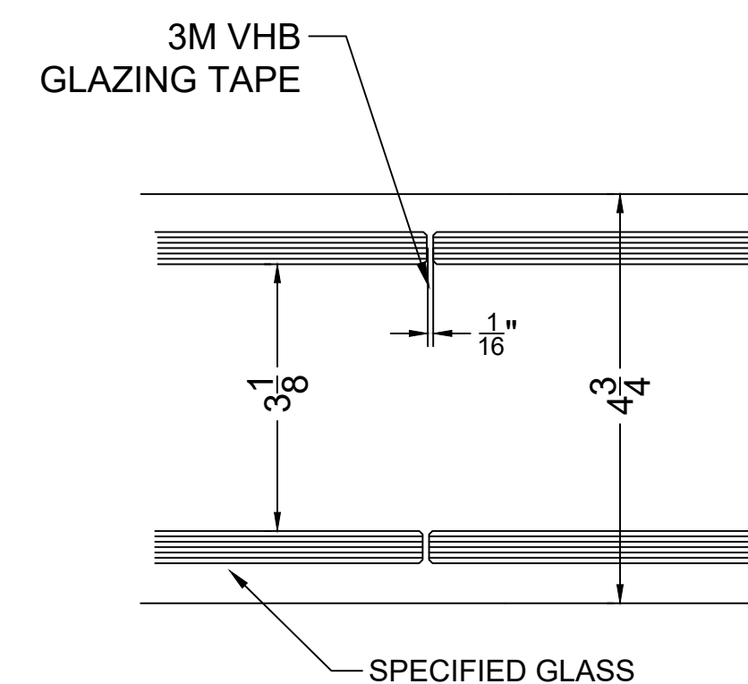
0 HORZ. SECT @ GLASS JOINT 49 STC
