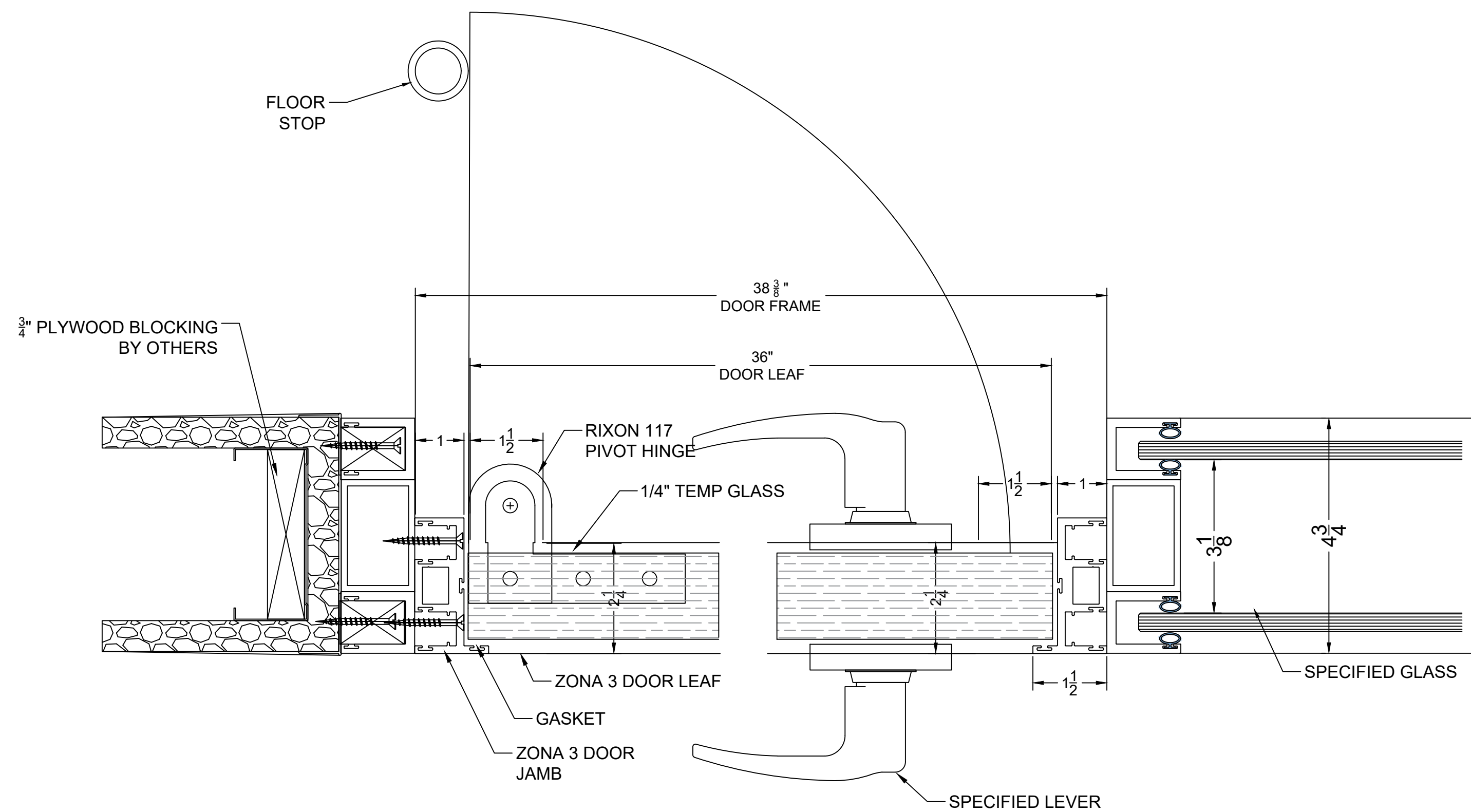
6A DOOR @ NIB WALL HORZ. SECT. @ WOOD DOOR W/LOCKSET 49 STC
