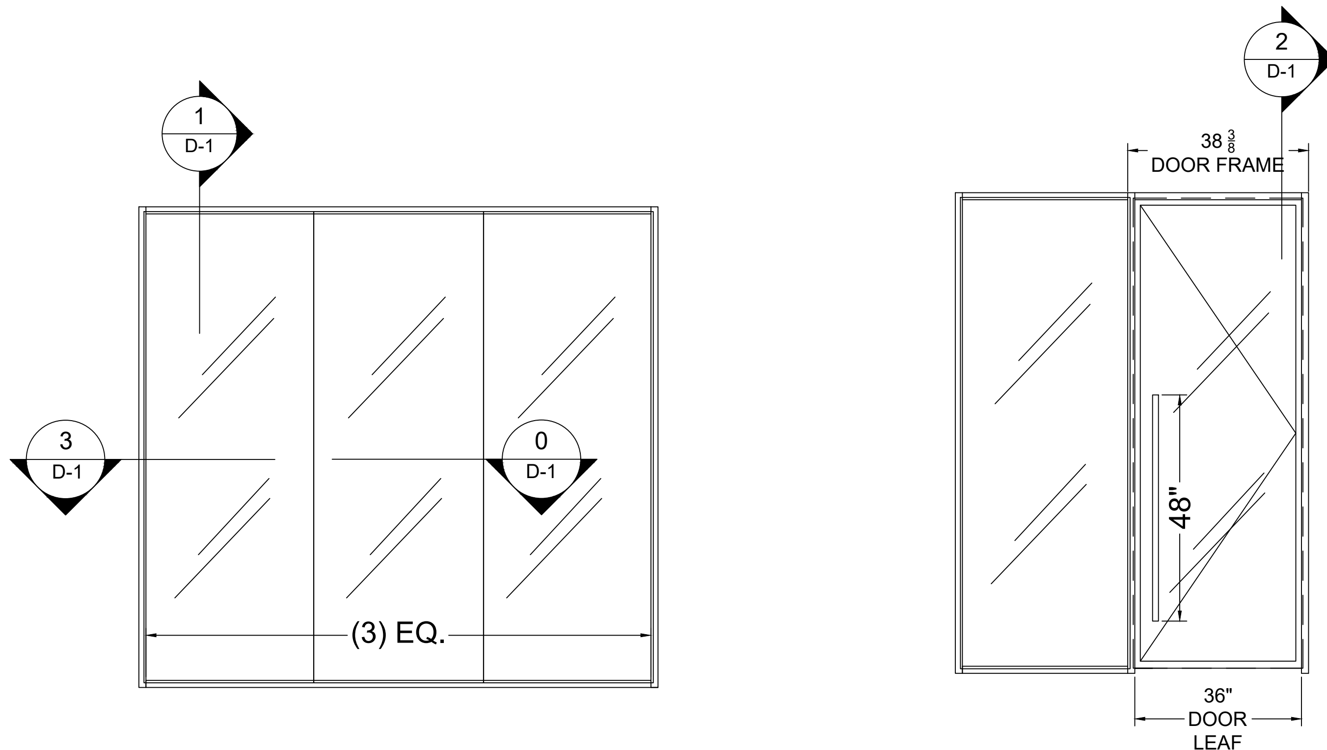
47 FIXED GLASS SYSTEM
