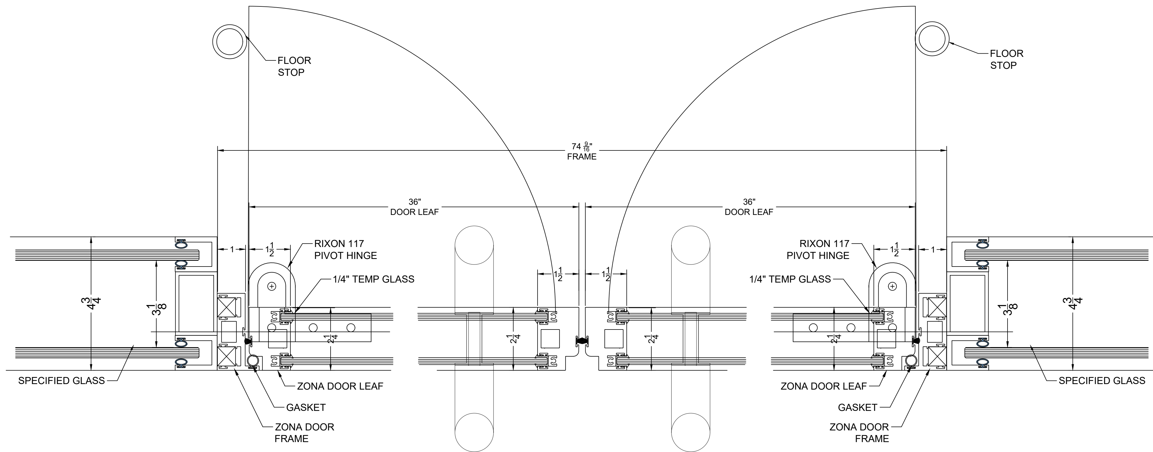
7 (2) ACTIVE DOORS BTW FIXED GLASS SIDE LITES HORZ. SECT. @ DBL GLZD DOUBLE DOORS W/PULL 49 STC
