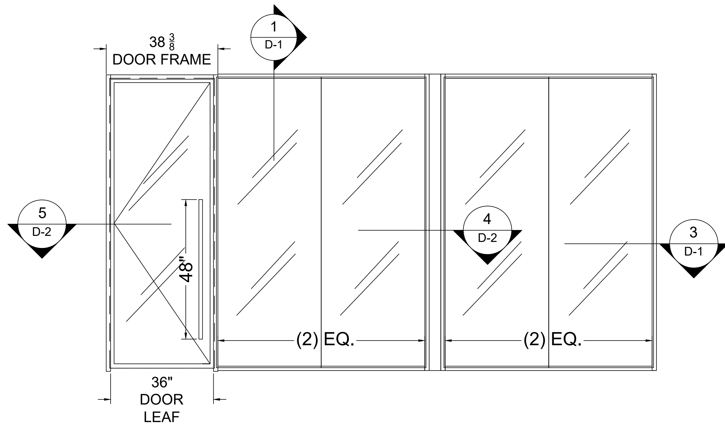
47 TYPICAL SYSTEM W/ DOOR STARTER AND DIVIDER
