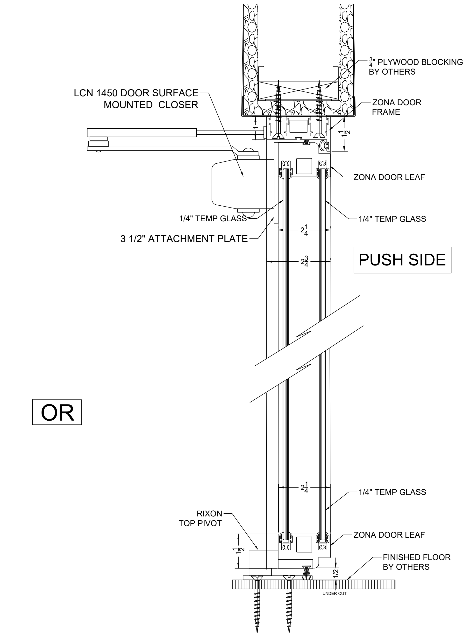
2 RIXON PIVOT HINGE- SURFACE MOUNTED CLOSER VERT. SECT. @ DBL GLZD DOOR
