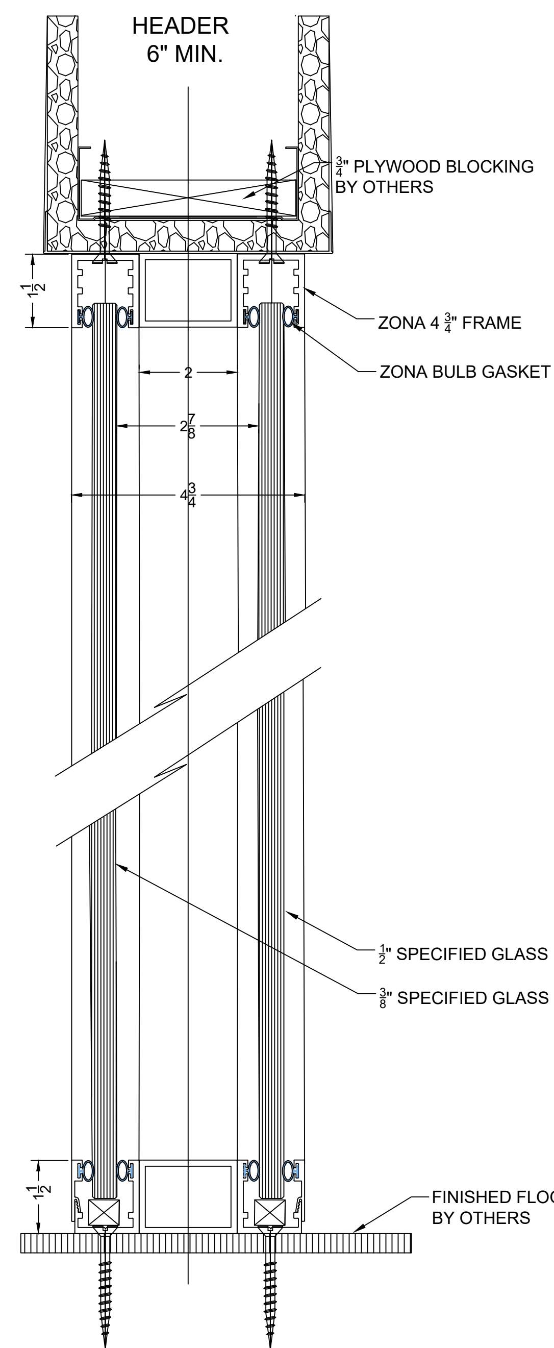
1 MAX. STC = 49 VERT. SECT @ ZONA DBL GLZD FIXED PANEL
