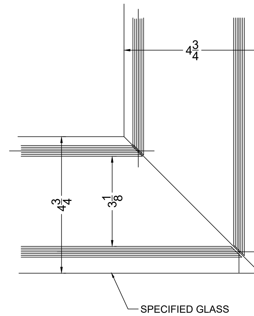
8 HORZ. SECT @ CORNER MITER 49 STC
