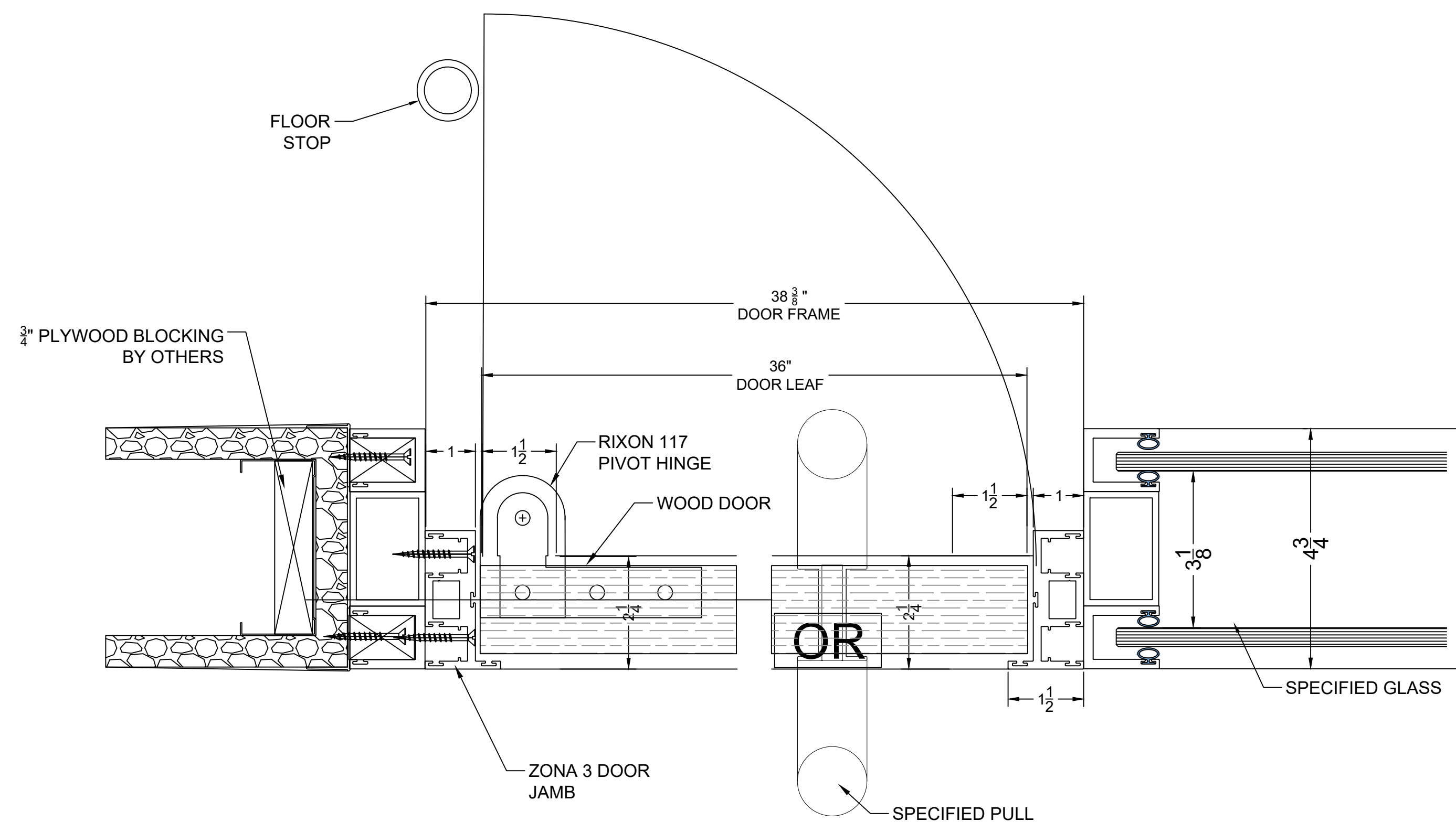
5A DOOR @ NIB WALL HORZ. SECT. @ WOOD DOOR W/PULL 49 STC
