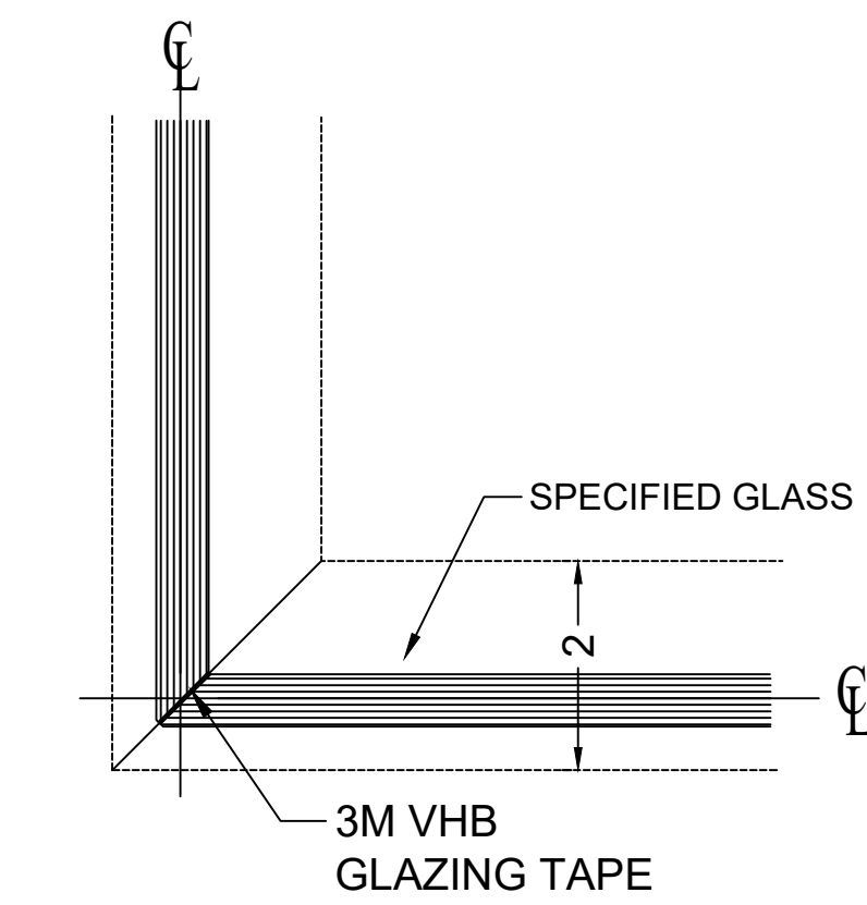
9 HORZ. SECT @ CORNER MITER
