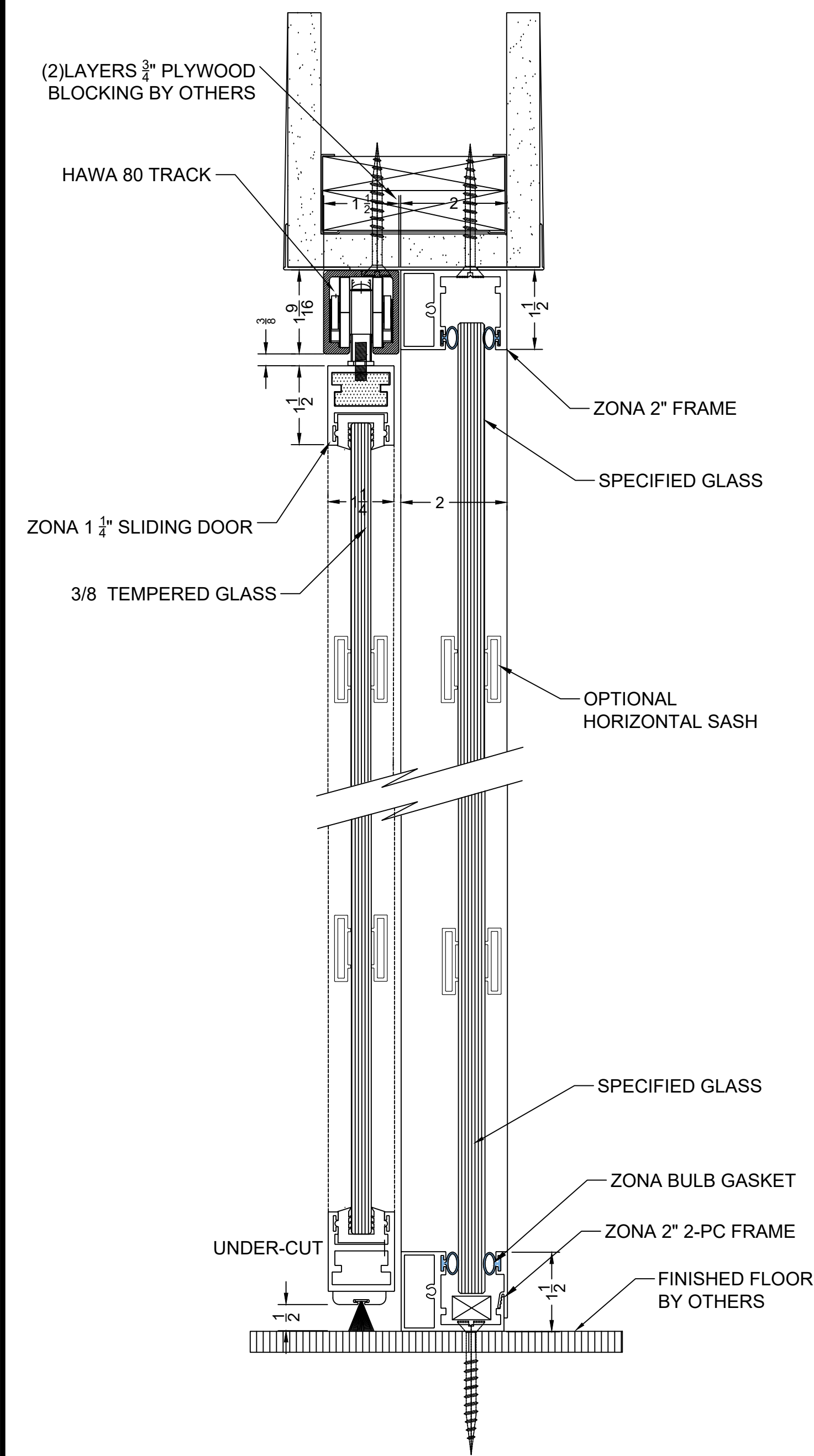
8 DIRECT MOUNT TRACK VERT. SECT @ SLIDING DOOR
