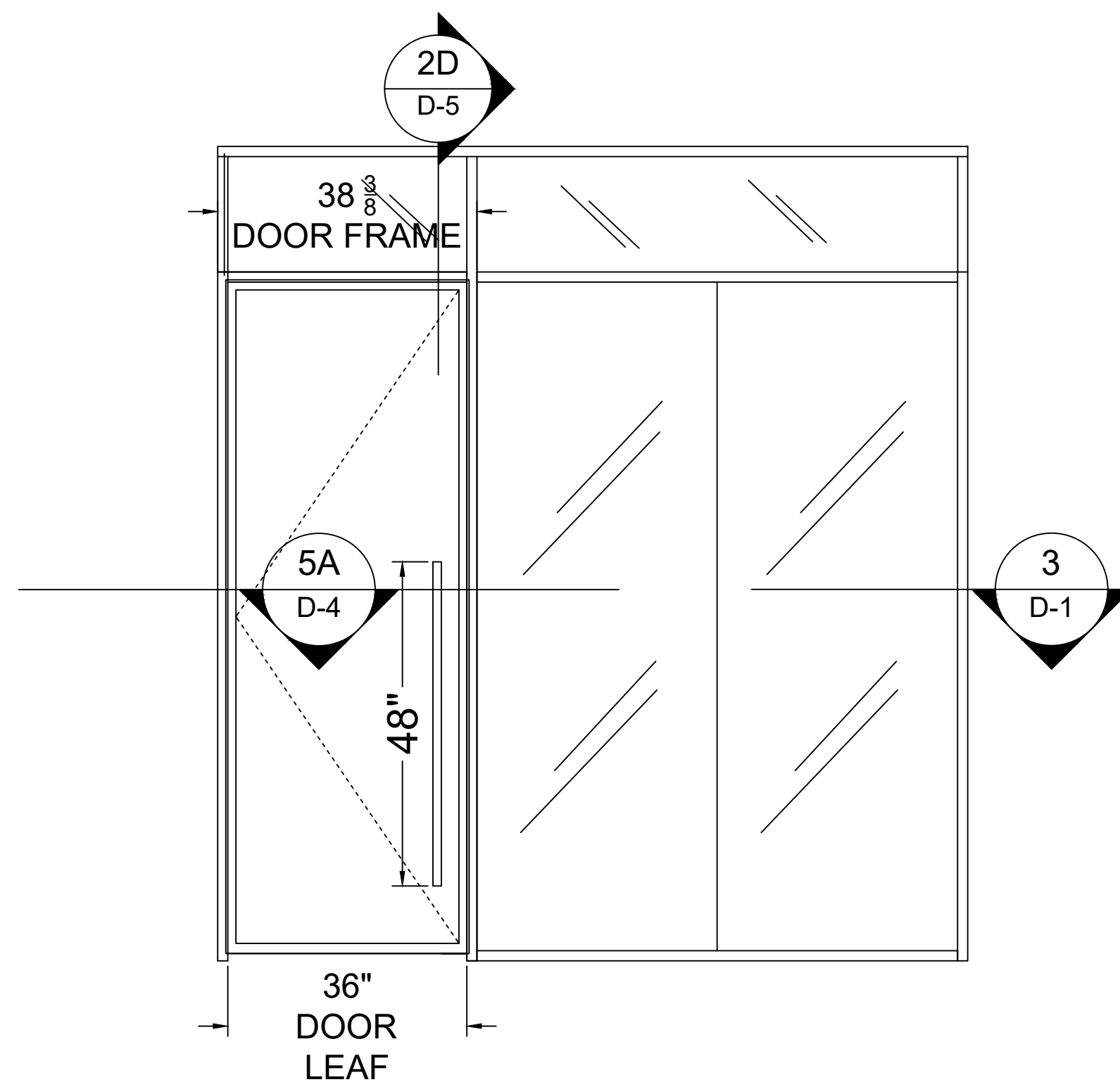
38 WOOD DOOR WITH CLERESTORY EXAMPLE
