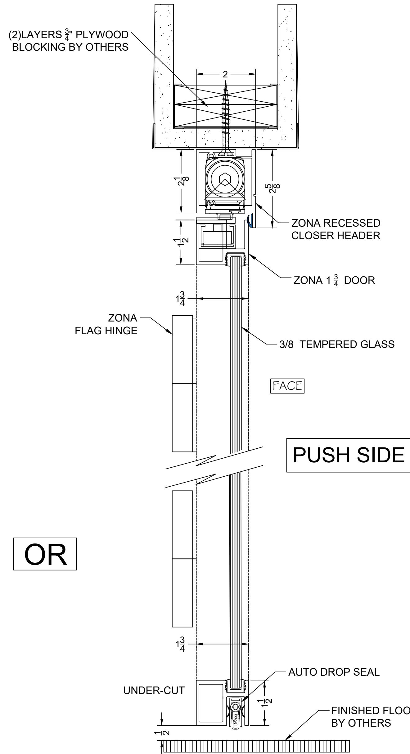
2 ZONA FLAG HINGE - RECESSED DOOR CLOSER VERT. SECT. @ DOOR
