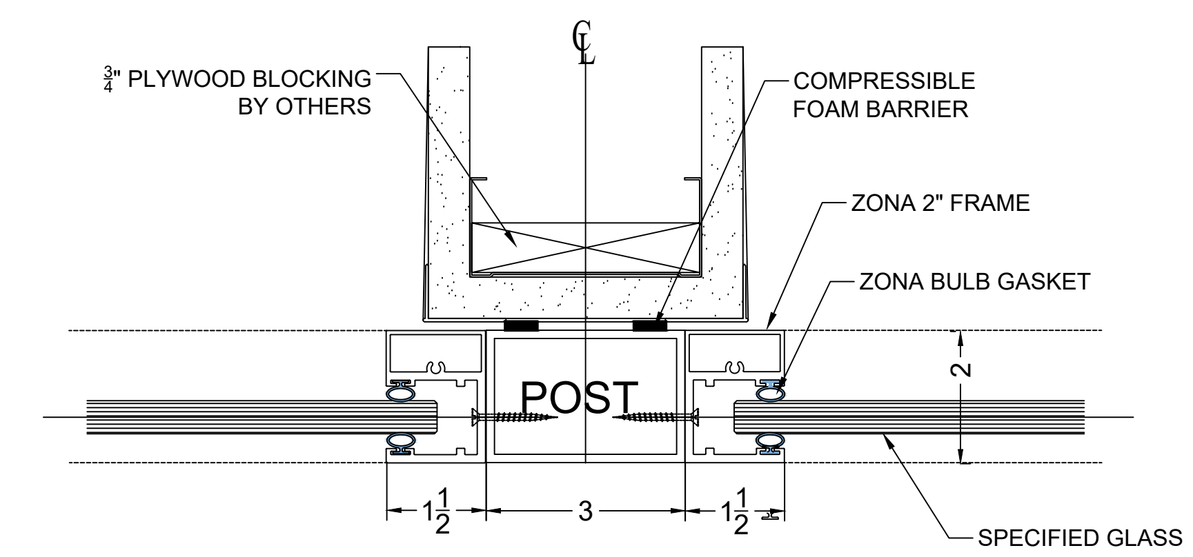
4 HORZ. SECT @ DIVIDER WALL WITH FLY-BY POST
