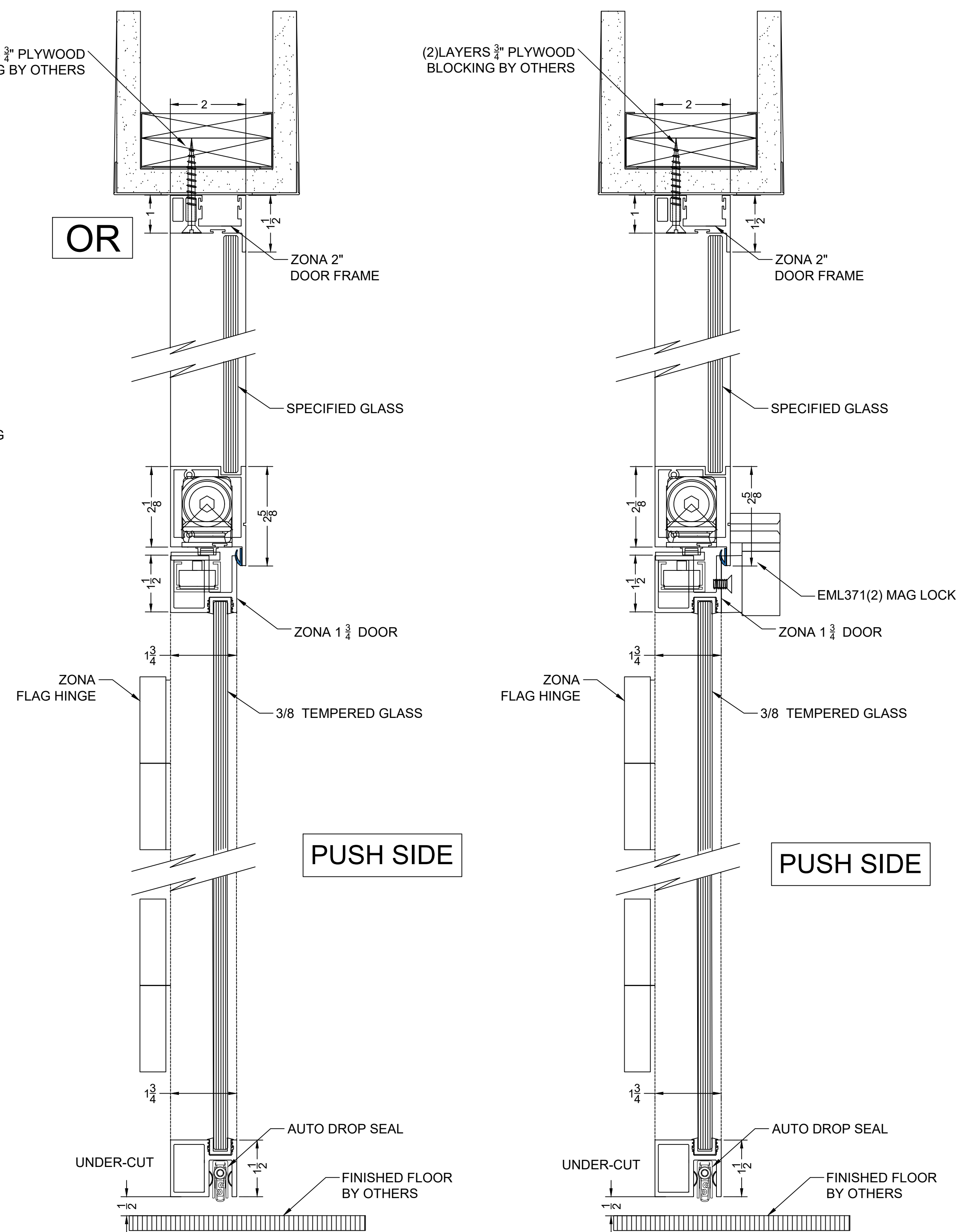
2 ZONA FLAG HINGE - CONCEALED CLOSER W/CLERESTORY VERT. SECT. @ DOOR
