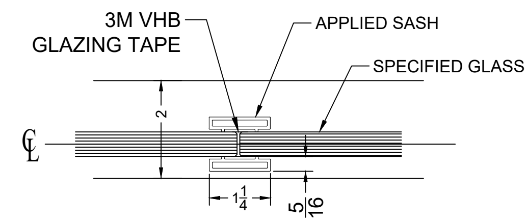
0B HORZ. SECT @ GLASS JOINT WITH VERTICAL SASH
