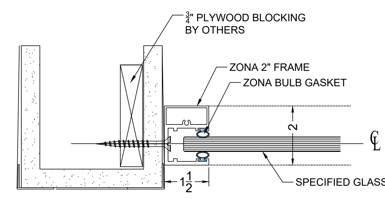
4 DIVIDER WALL HORZ. SECT @ FIXED PANEL @ DIVIDER WALL
