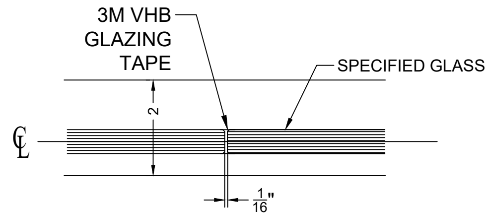
0 HORZ. SECT @ GLASS JOINT
