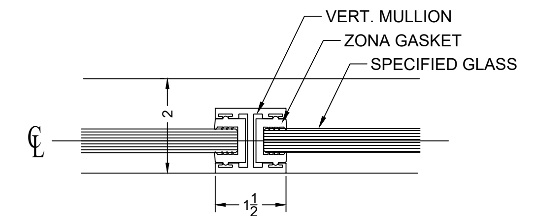
0B HORZ. SECT @ GLASS JOINT WITH VERTICAL MULLION
