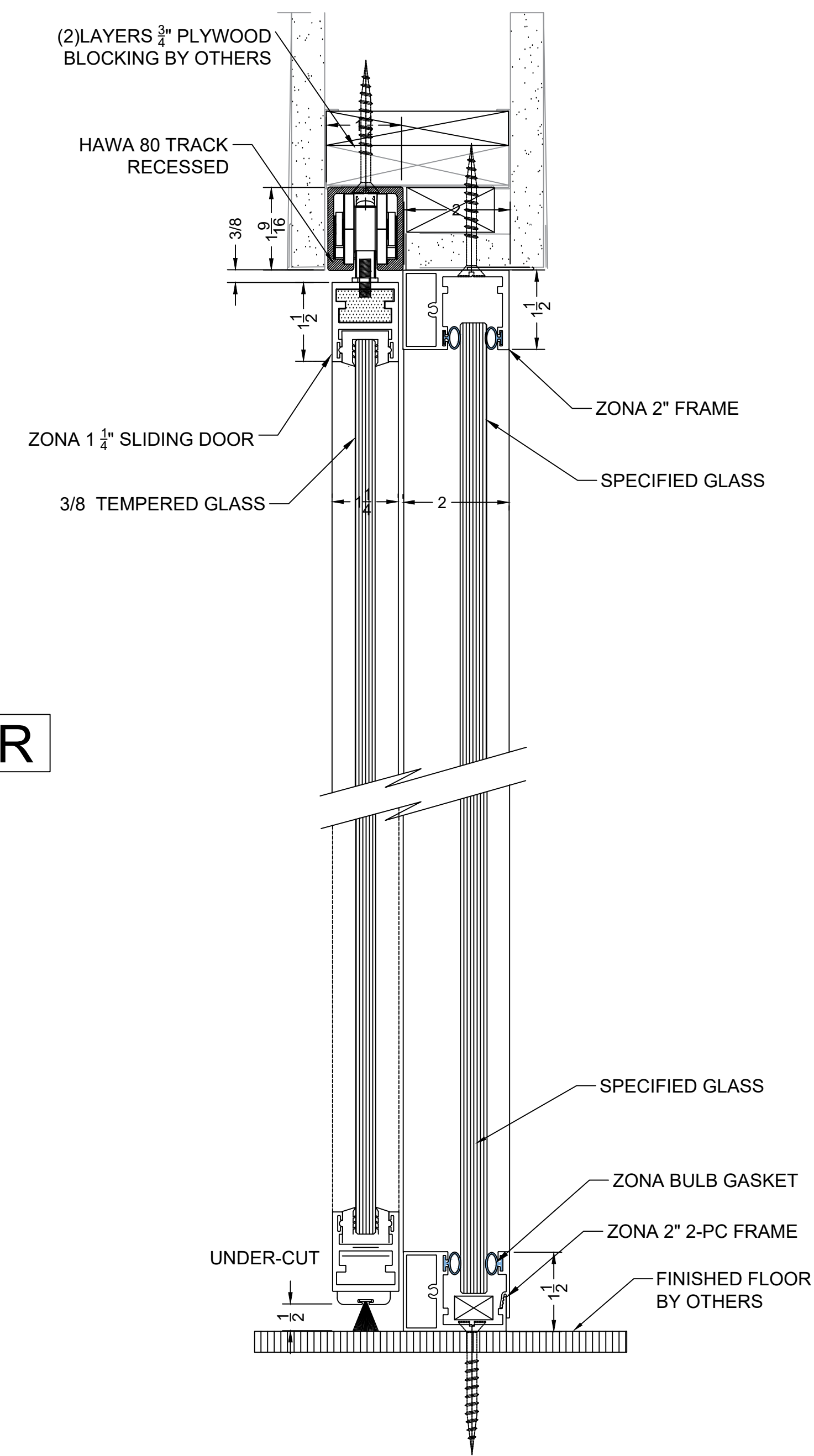
8 RECESSED TRACK MOUNT VERT. SECT @ SLIDING DOOR
