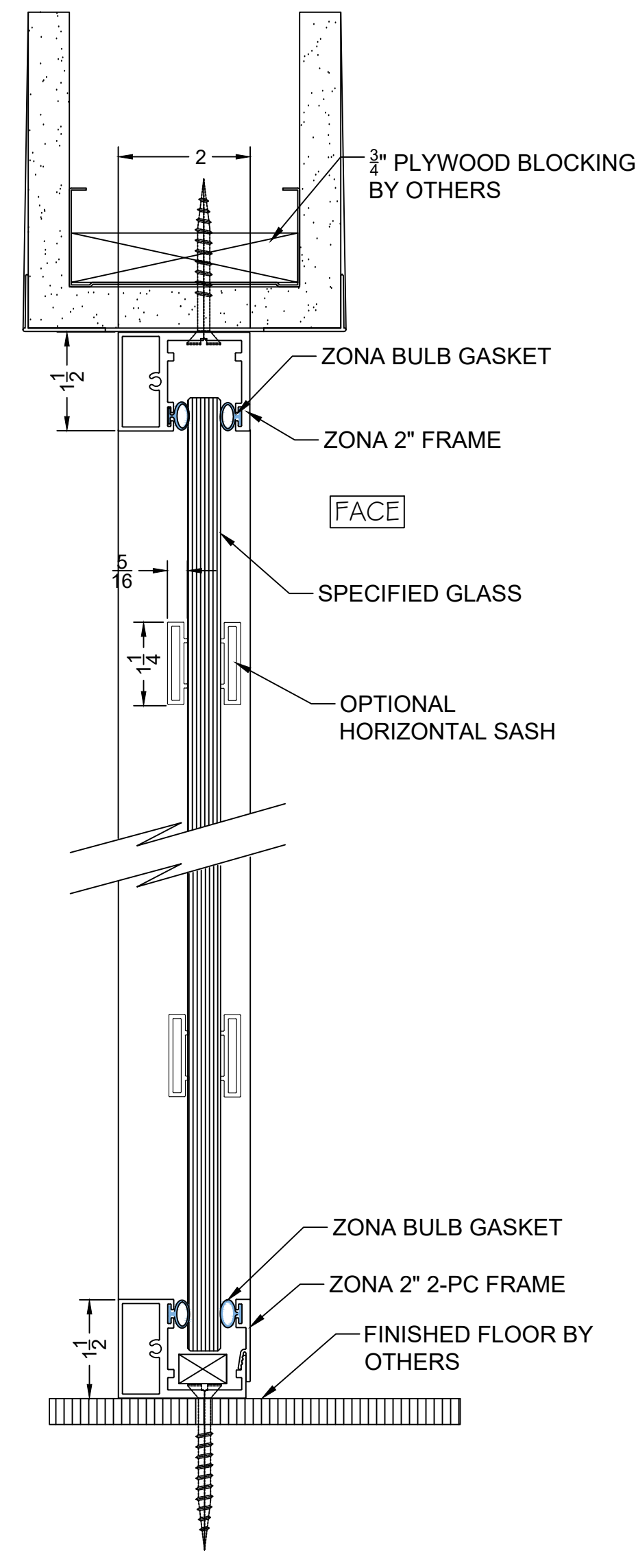
1 VERT. SECT @ ZONA FIXED PANEL
