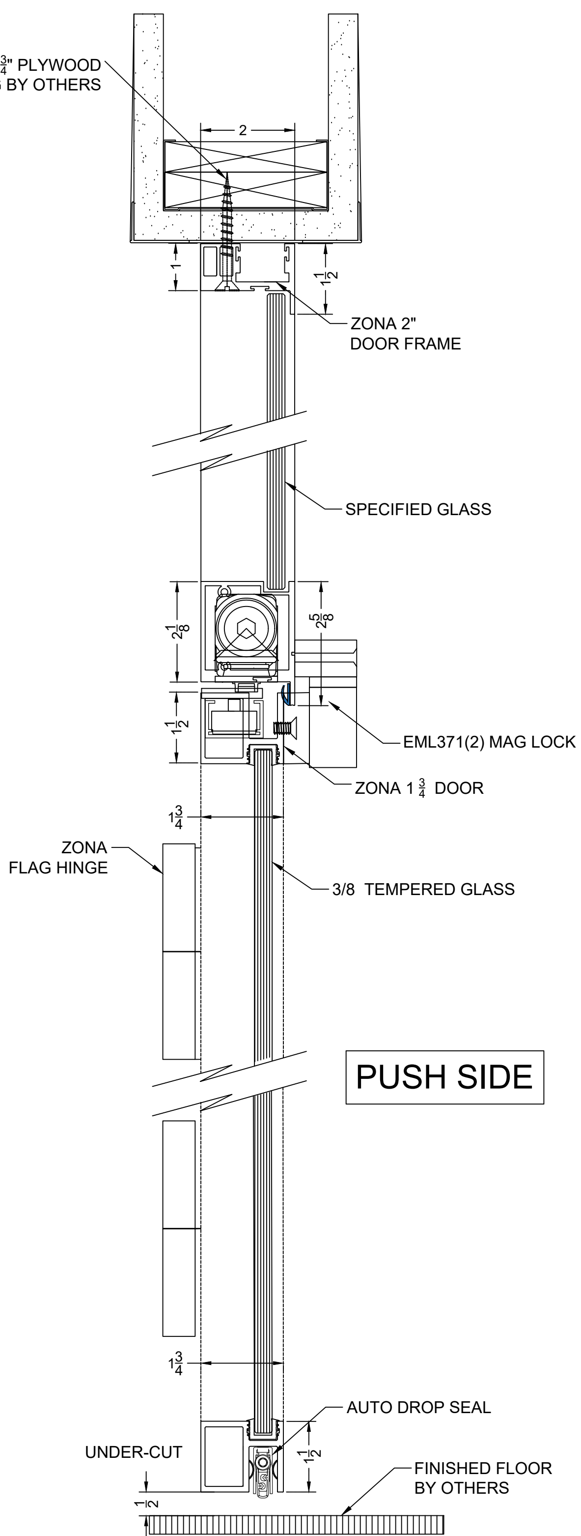
2 ZONA FLAG HINGE - CONCEALED CLOSER W/CLERESTORY VERT. SECT. @ DOOR
