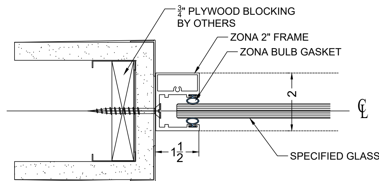
3 SECTION @ FIXED PANEL @ WALL
