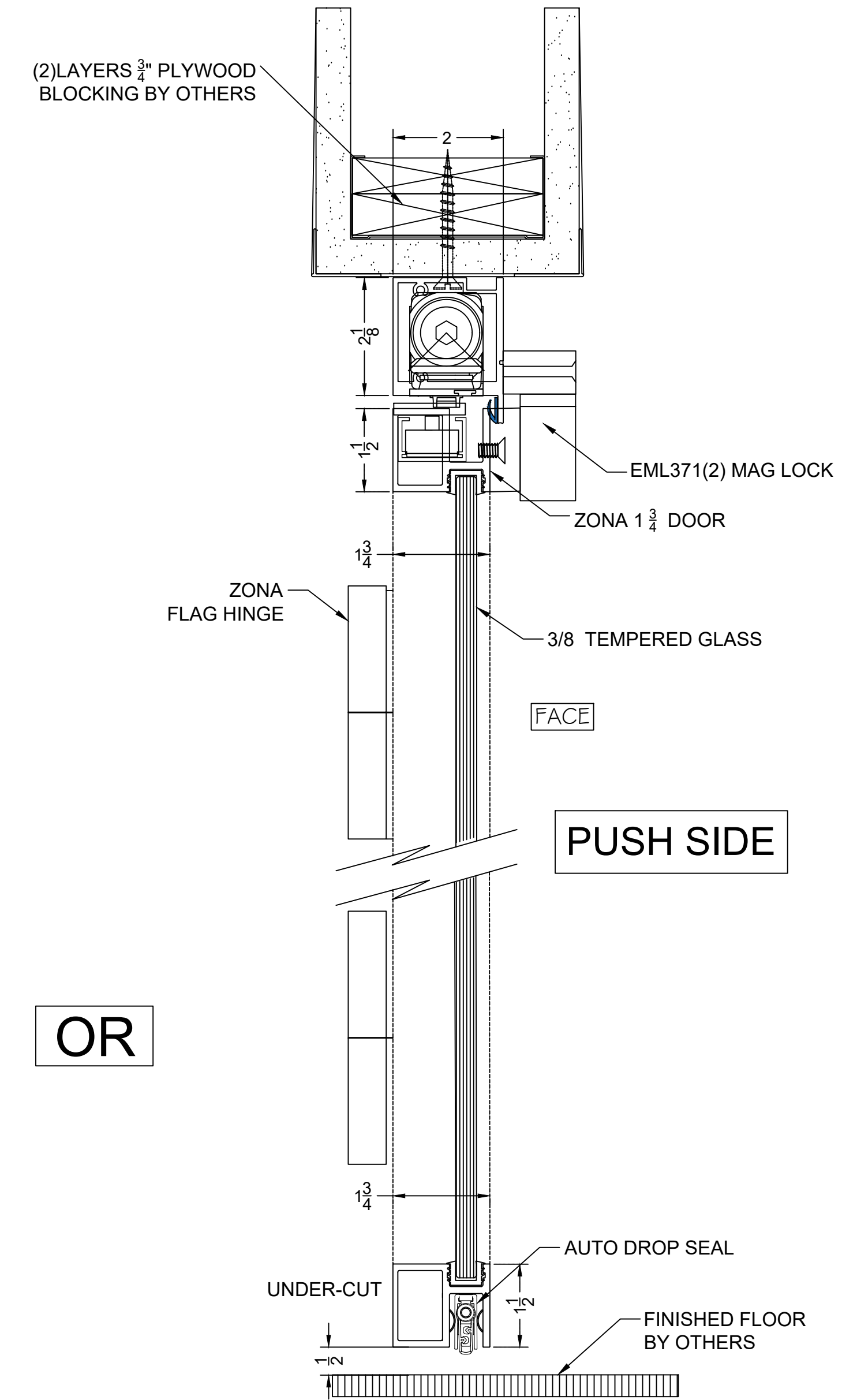
2 ZONA FLAG HINGE - SECURED DOOR VERT. SECT. @ DOOR
