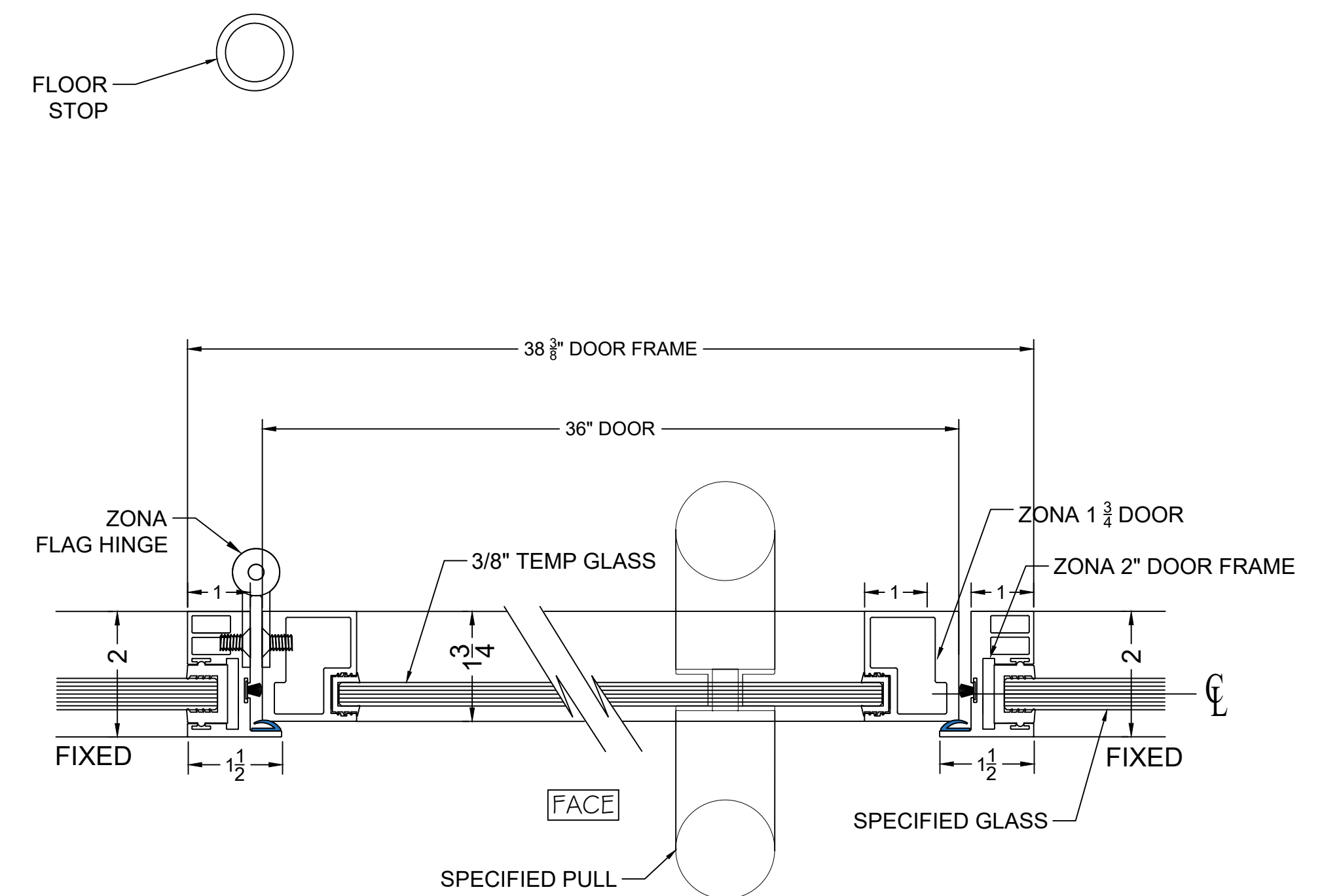
6 DOOR BTW FIXED GLASS PANELS HORZ. SECT. @ DOOR W/PULL
