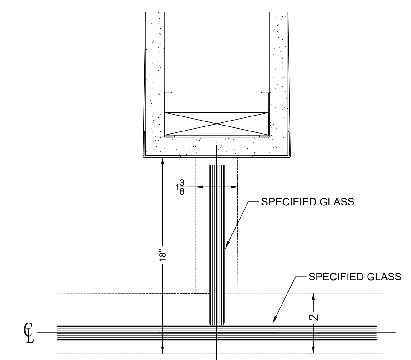
4 HORZ. SECT @ "T" CONNECTION
