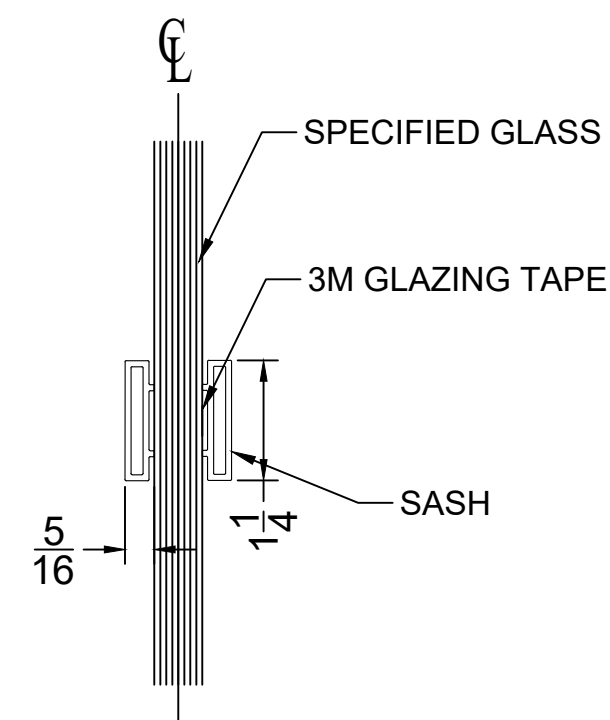
0A VERT. SECTION @ GLASS JOINT WITH HORZ. SASH
