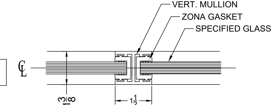
0B HORZ. SECT @ GLASS JOINT WITH VERTICAL MULLION
