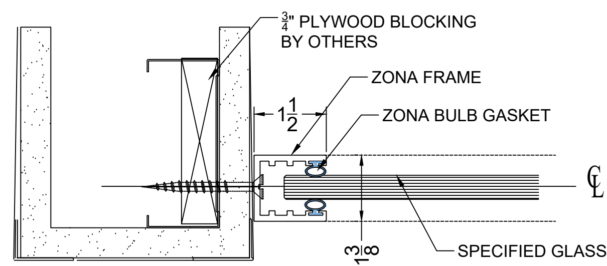
6 HORZ. SECT @ FIXED PANEL @ WALL DIVIDER WALL
