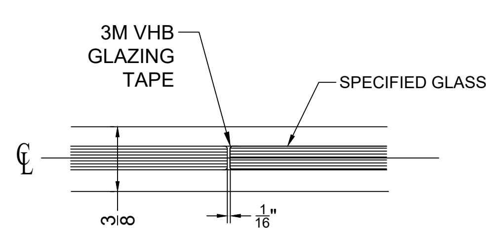
0 HORZ. SECT @ GLASS JOINT CRL VHB GLAZING TAPE
