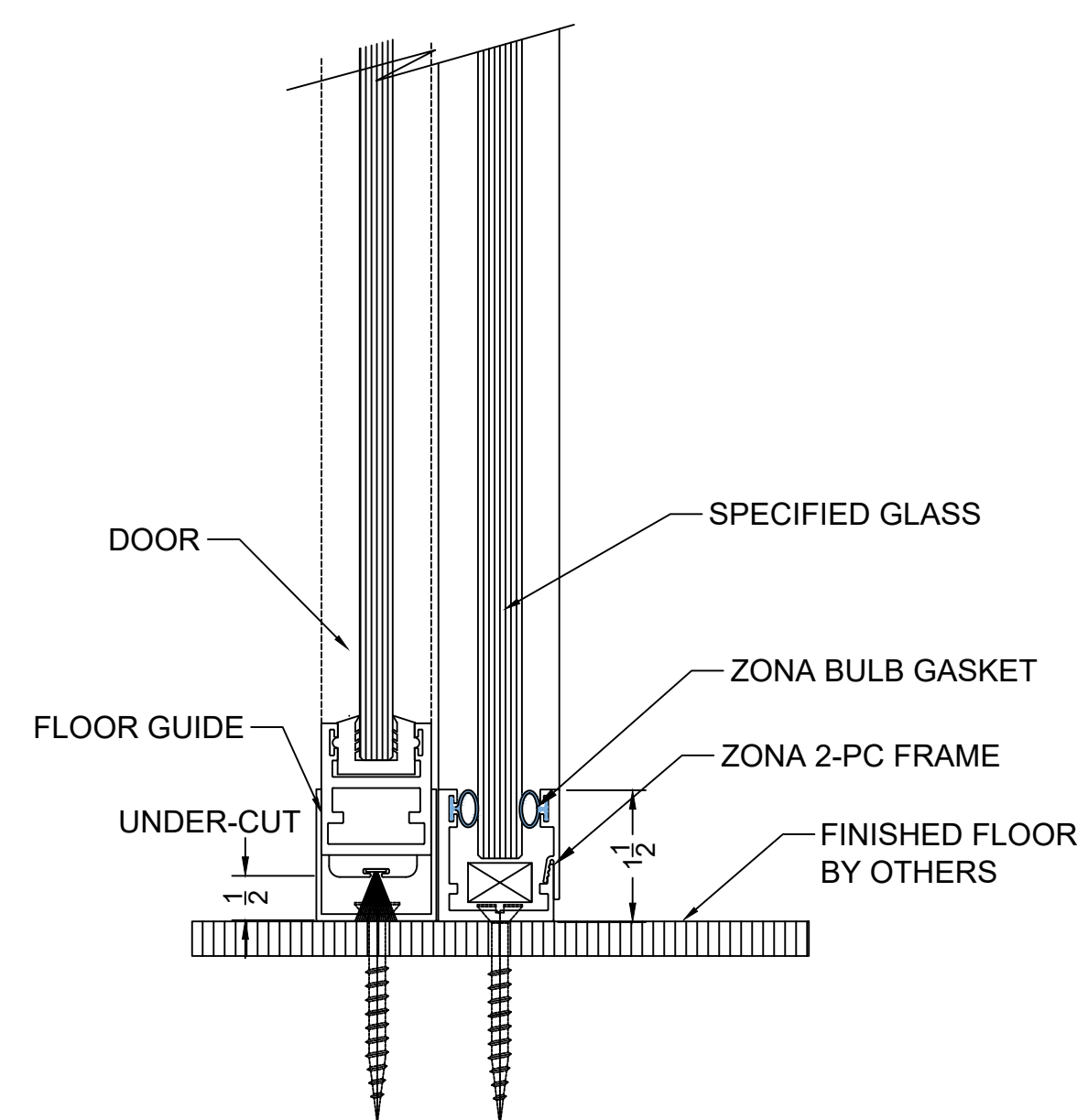
8 RECESSED TRACK MOUNT VERT. SECT @ SLIDING DOOR
