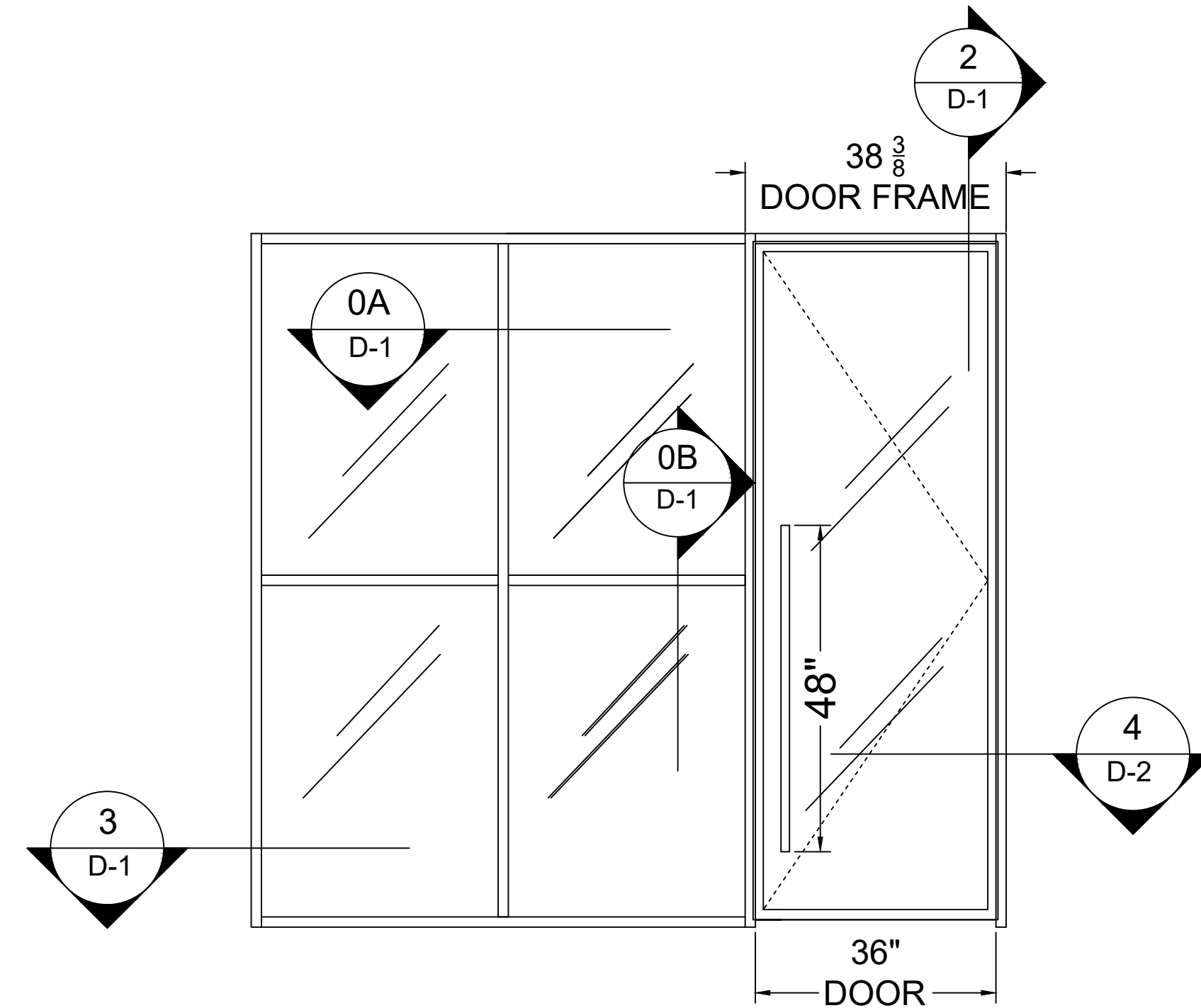
Z1 SASH OFFICE FRONT EXAMPLE
