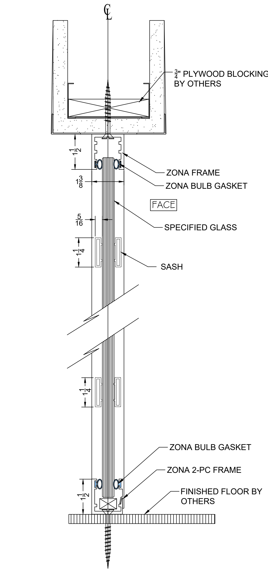
3 VERT. SECT @ ZONA FIXED PANEL WITH SASH
