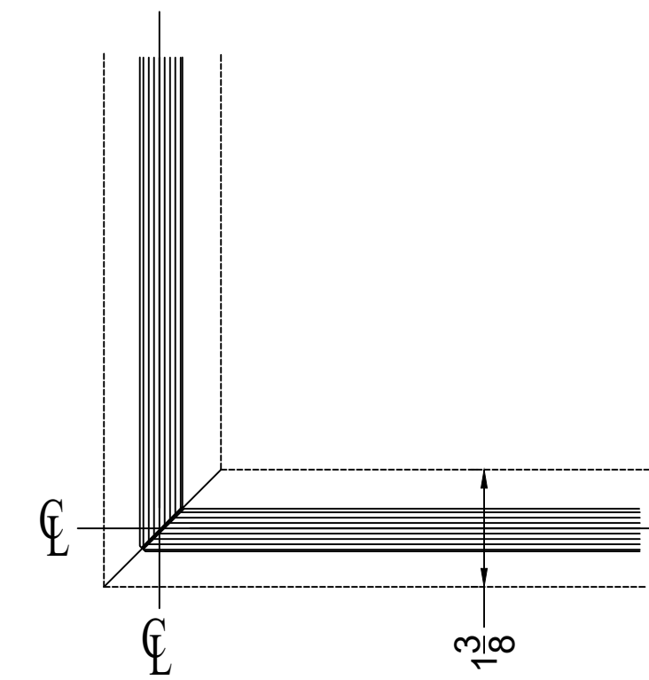
10 HORZ. SECT @ CORNER MITER
