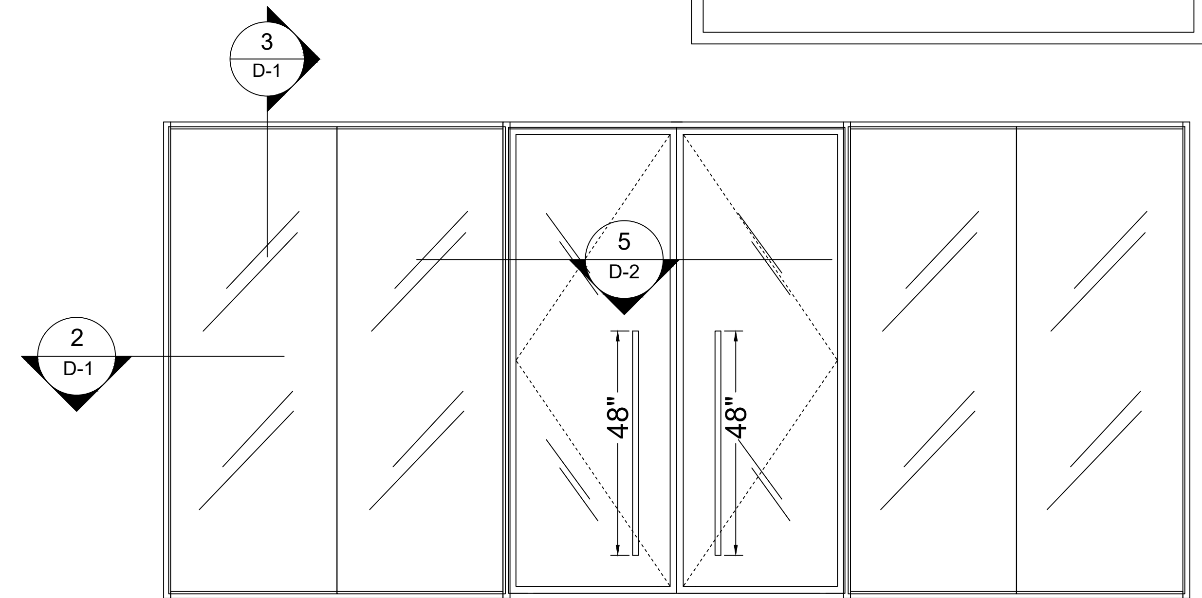
Z1 DOUBLE DOOR WITH FIXED GLASS EXAMPLE
