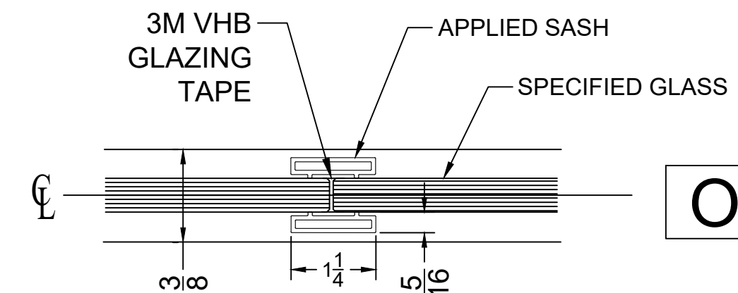
0B HORZ. SECT @ GLASS JOINT WITH VERTICAL SASH
