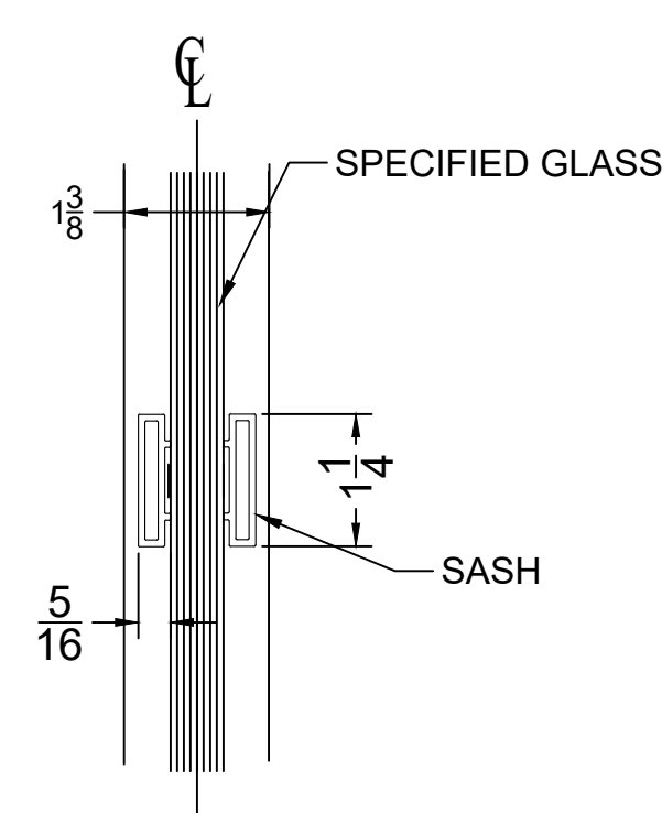
0A VERT. SECTION @ GLASS JOINT WITH HORZ. SASH
