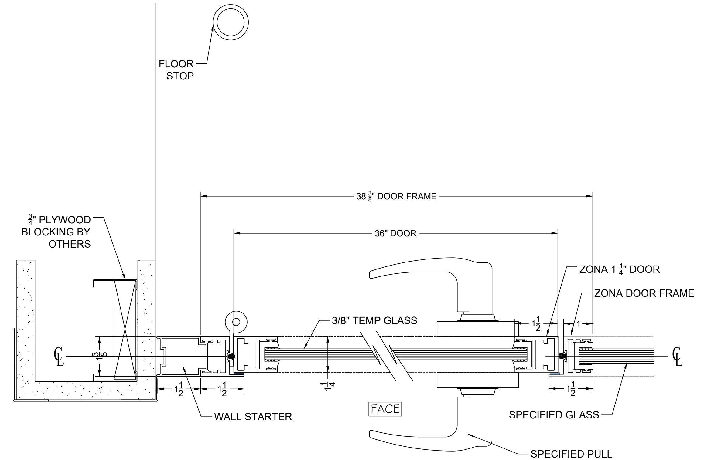
7 LEVER & LOCKSET @ DIVIDING WALL HORZ. SECT. @ DOOR
