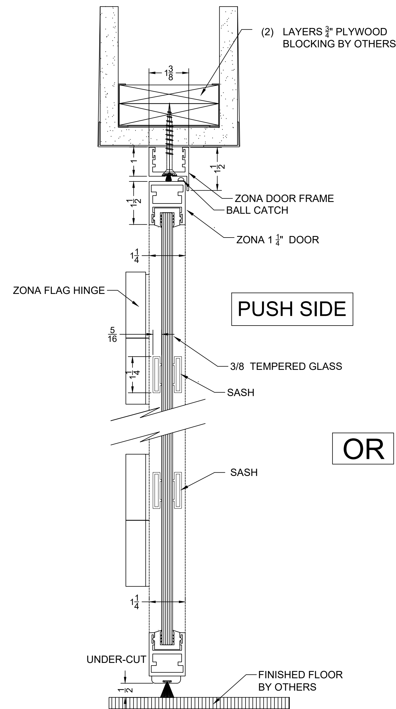
1 ZONA FLAG HINGE - FREE-SWING DOOR VERT. SECT. @ DOOR W/SASH
