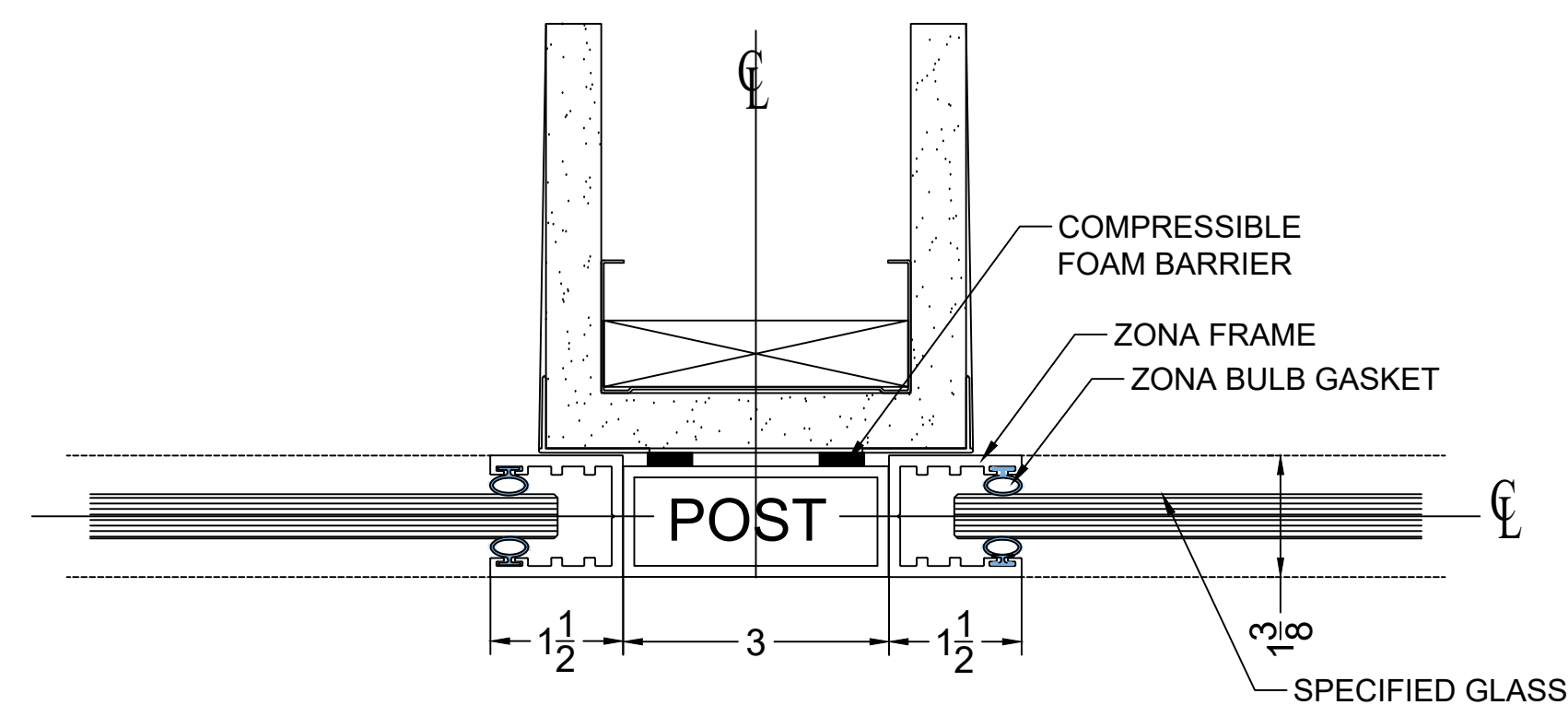
6 HORZ. SECT @ DIVIDER WALL WITH FLY-BY POST
