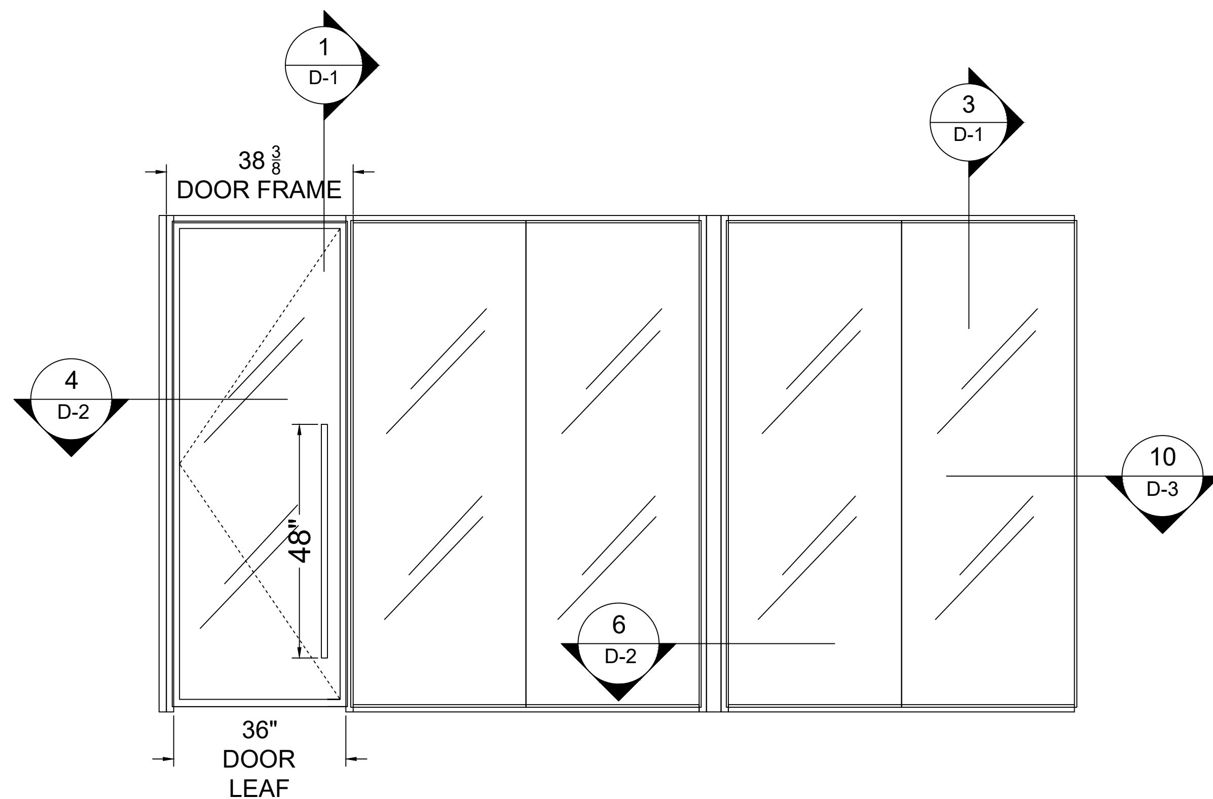
Z1 TYPICAL SYSTEM W/ DOOR STARTER & SASH EXAMPLE
