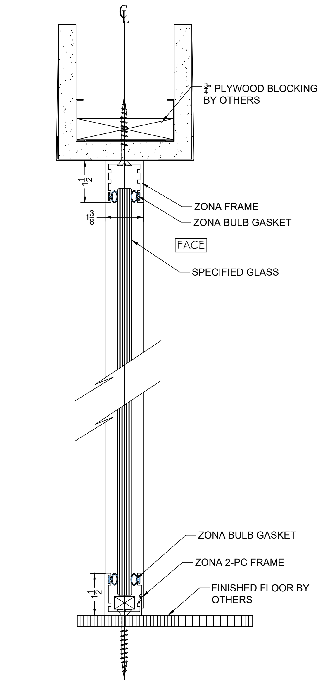
3 VERT. SECT @ ZONA FIXED PANEL WITHOUT SASH
