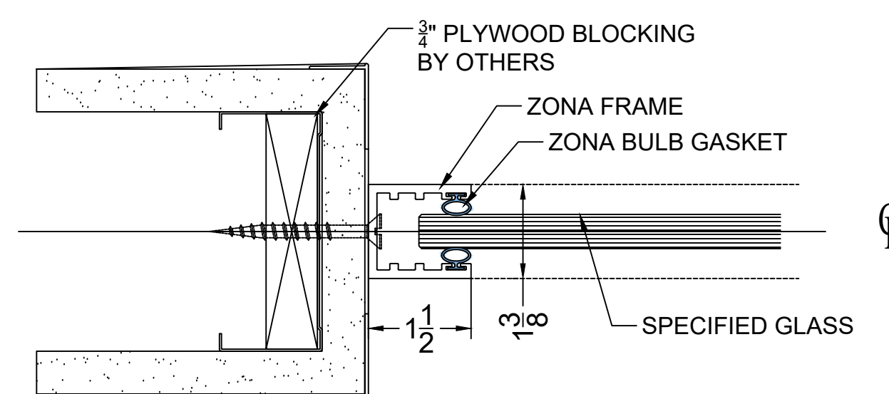
2 SECTION @ FIXED PANEL @ WALL
