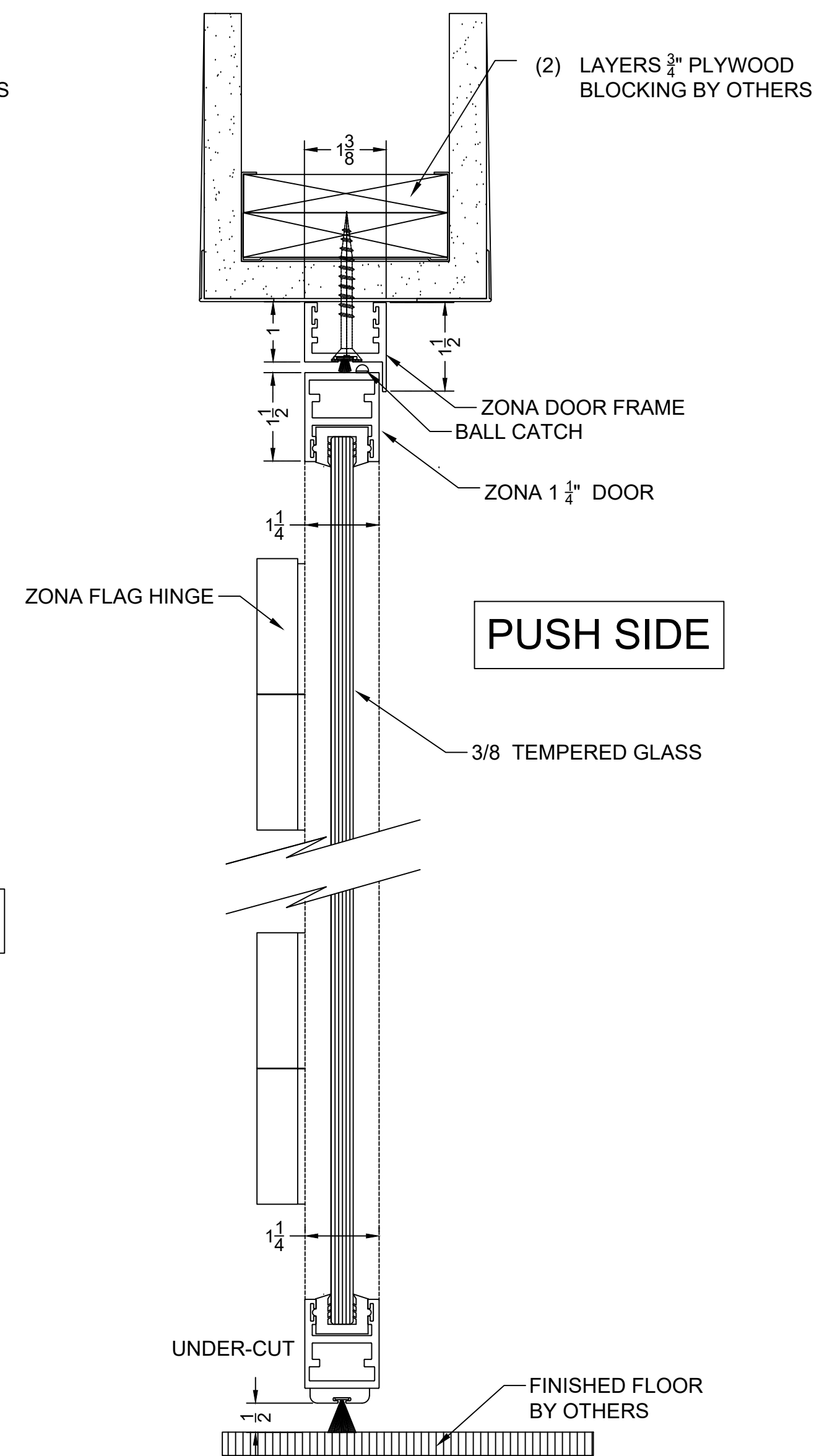
1 ZONA FLAG HINGE - FREE-SWING DOOR VERT. SECT. @ DOOR W/O SASH
