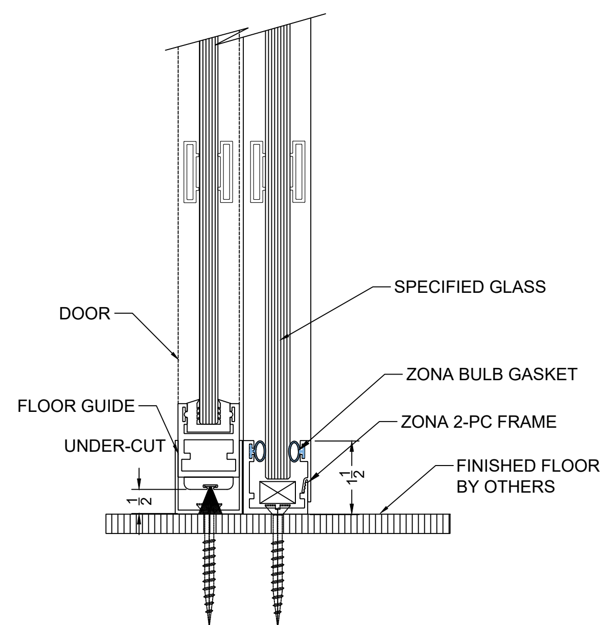
8 DIRECT MOUNT TRACK VERT. SECT @ SLIDING DOOR
