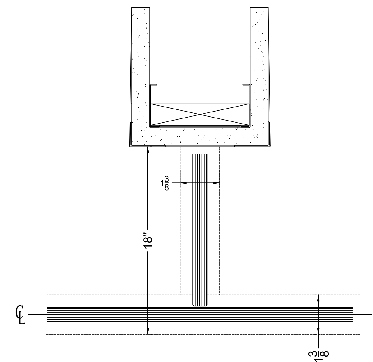
6 HORZ. SECT @ "T" CONNECTION
